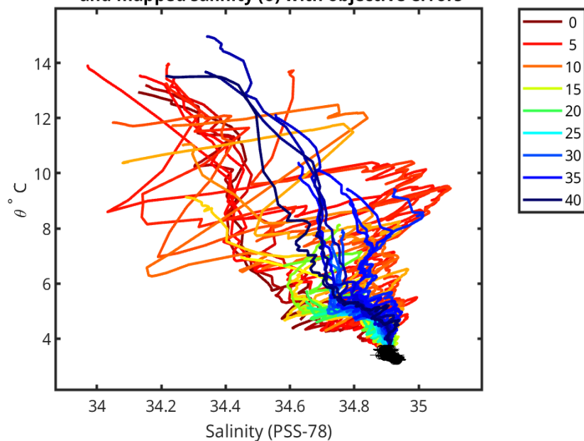
5907202 uncalibrated float data (-) and mapped salinity (o) with objective errors
