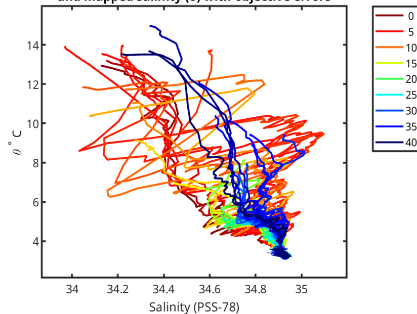
5907202 calibrated float data (-) and mapped salinity (o) with objective errors
