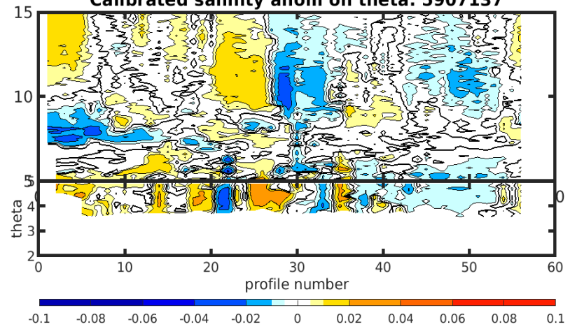
Calibrated salinity anom on theta. 5907137
