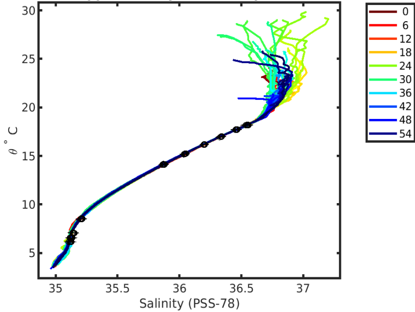
5907137 uncalibrated float data (-) and mapped salinity (o) with objective errors
