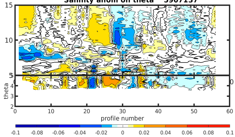
Salinity anom on theta 5907137
