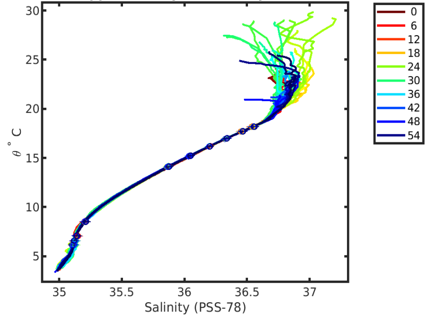
5907137 calibrated float data (-) and mapped salinity (o) with objective errors
