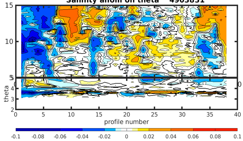
Salinity anom on theta 4903831
