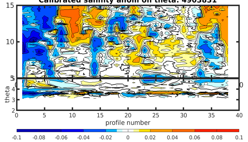
Calibrated salinity anom on theta. 4903831
