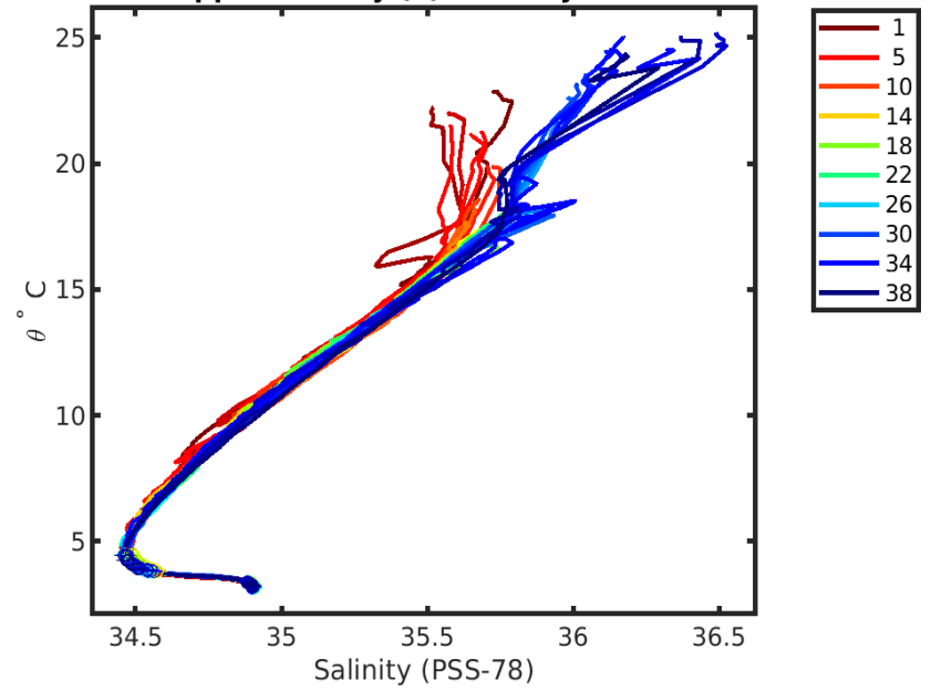
4903831 calibrated float data (-) and mapped salinity (o) with objective errors
