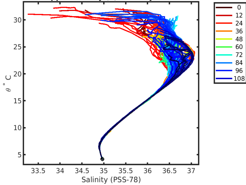
4903552 uncalibrated float data (-) and mapped salinity (o) with objective errors
