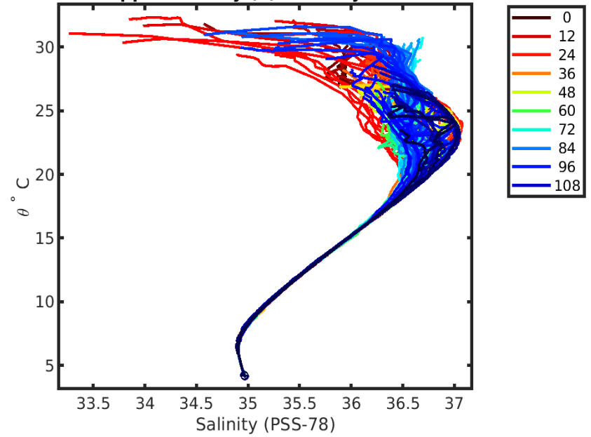
4903552 calibrated float data (-) and mapped salinity (o) with objective errors
