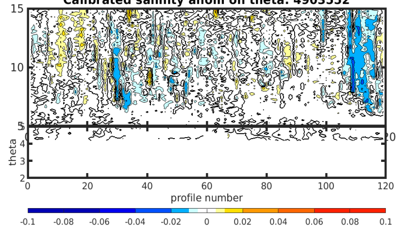
Calibrated salinity anom on theta. 4903552
