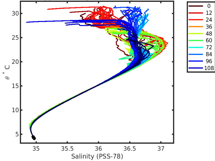
4903547 uncalibrated float data (-) and mapped salinity (o) with objective errors
