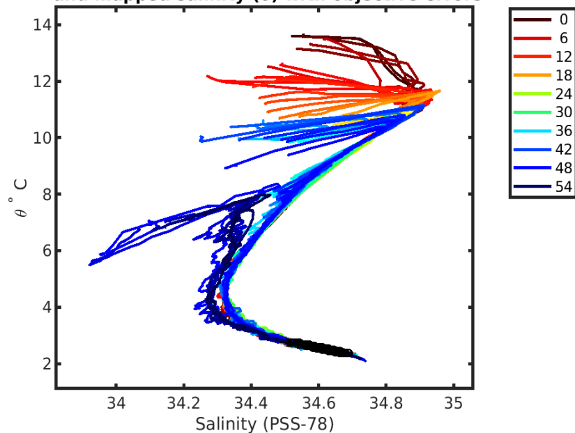
4903482 uncalibrated float data (-) and mapped salinity (o) with objective errors
