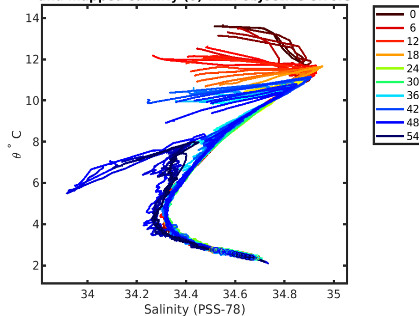
4903482 calibrated float data (-) and mapped salinity (o) with objective errors
