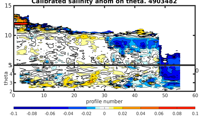
Calibrated salinity anom on theta. 4903482
