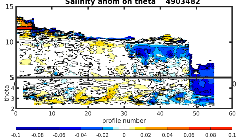
Salinity anom on theta 4903482
