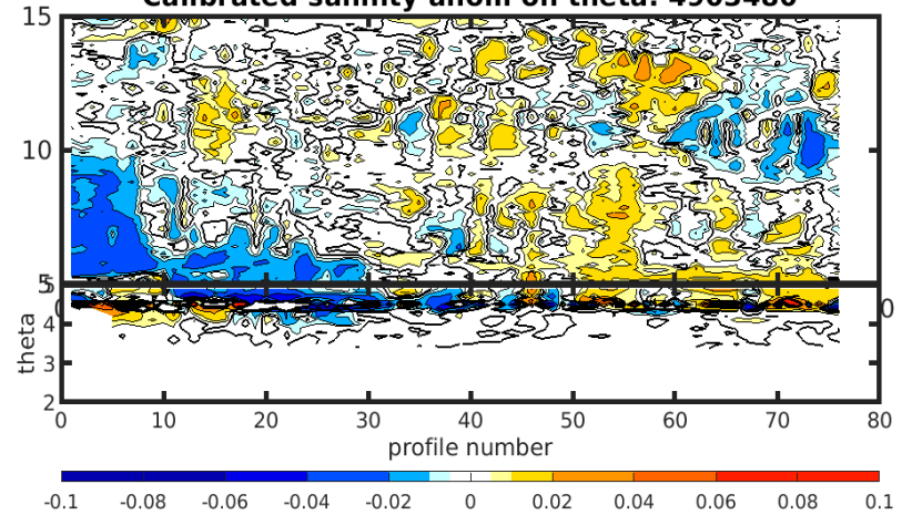
Calibrated salinity anom on theta. 4903480
