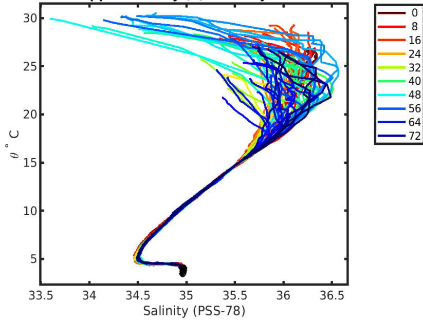
4903480 uncalibrated float data (-) and mapped salinity (o) with objective errors
