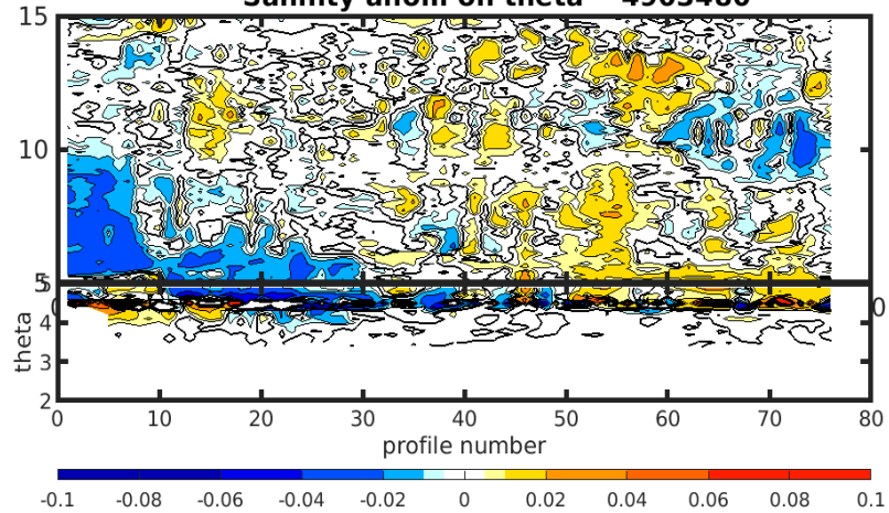
Salinity anom on theta 4903480
