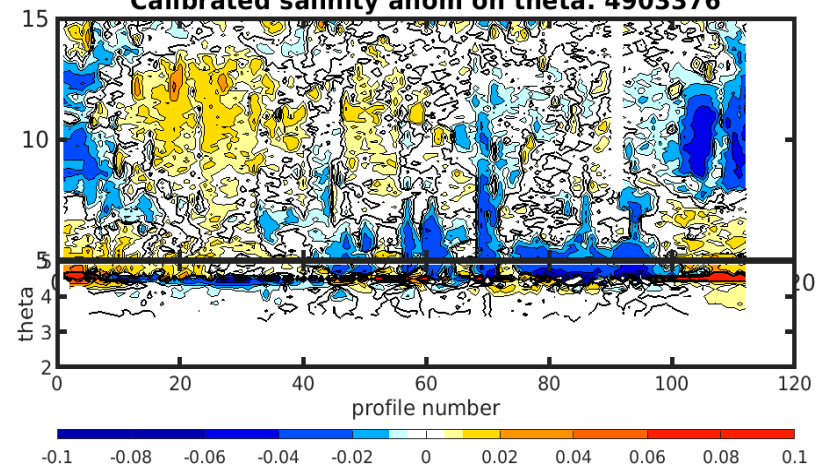
Calibrated salinity anom on theta. 4903376
