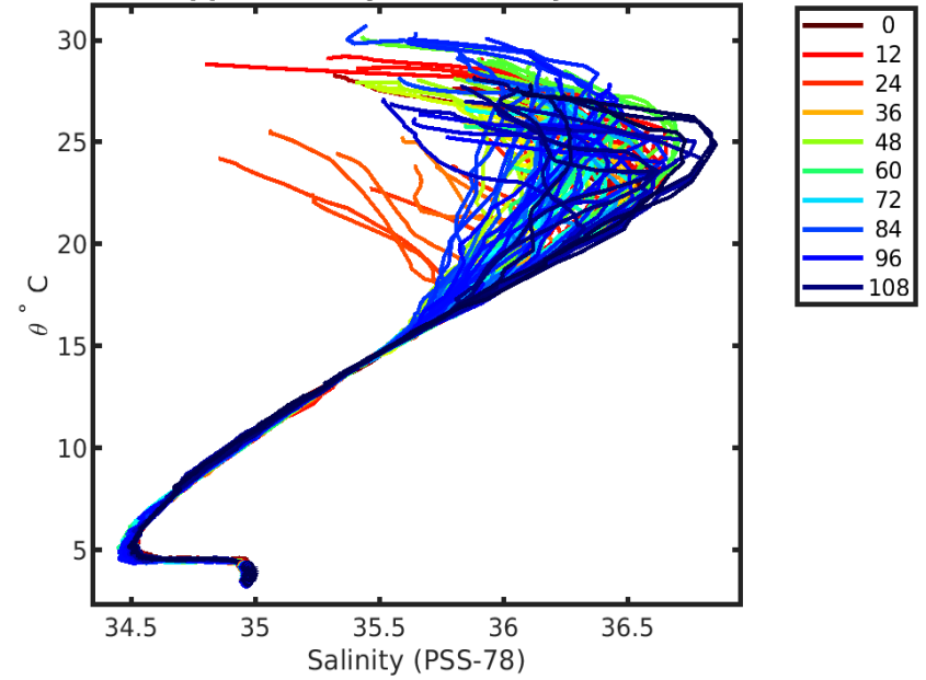
4903376 calibrated float data (-) and mapped salinity (o) with objective errors
