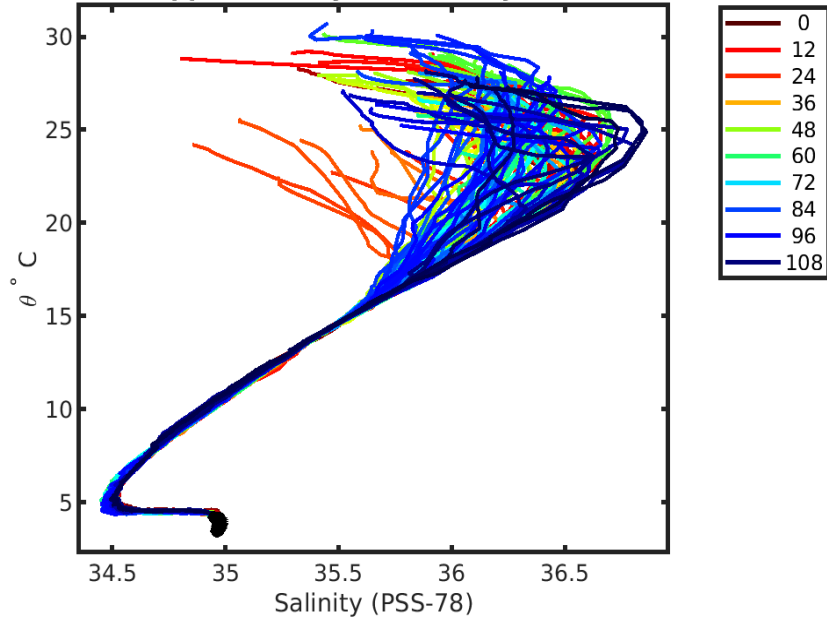
4903376 uncalibrated float data (-) and mapped salinity (o) with objective errors
