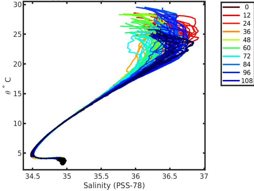
4903367 uncalibrated float data (-) and mapped salinity (o) with objective errors
