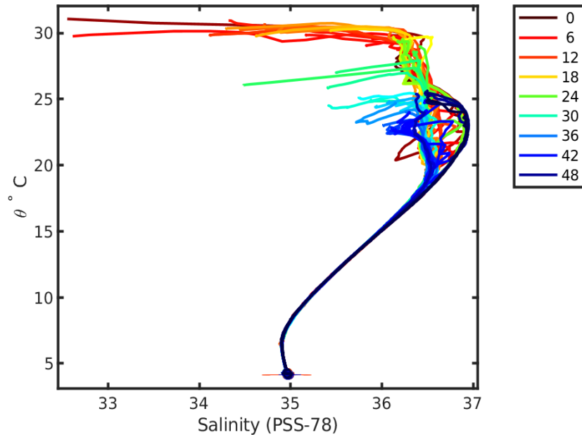
4903235 calibrated float data (-) and mapped salinity (o) with objective errors
