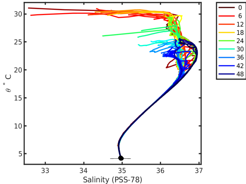
4903235 uncalibrated float data (-) and mapped salinity (o) with objective errors
