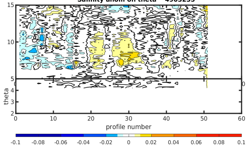
Salinity anom on theta 4903235
