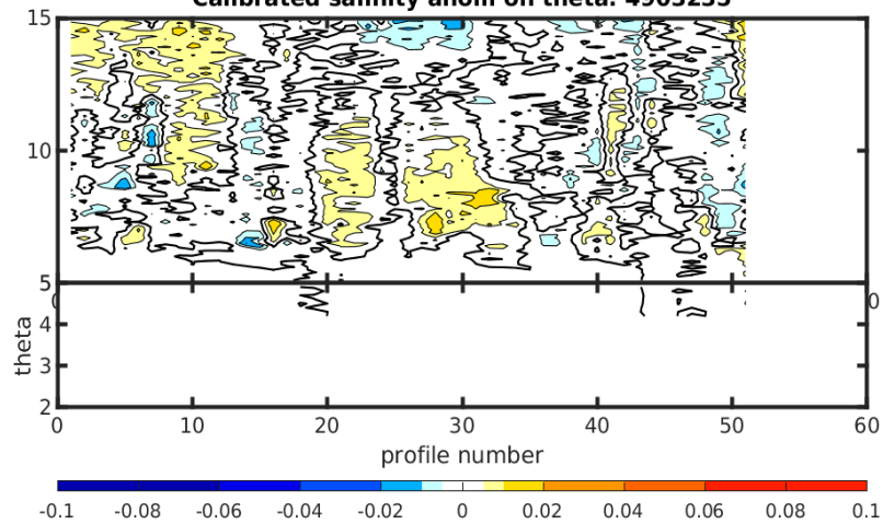
Calibrated salinity anom on theta. 4903235
