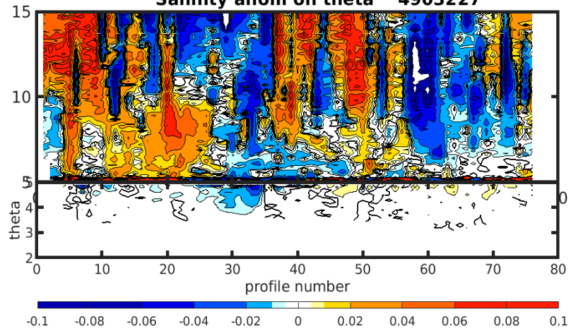
Salinity anom on theta 4903227
