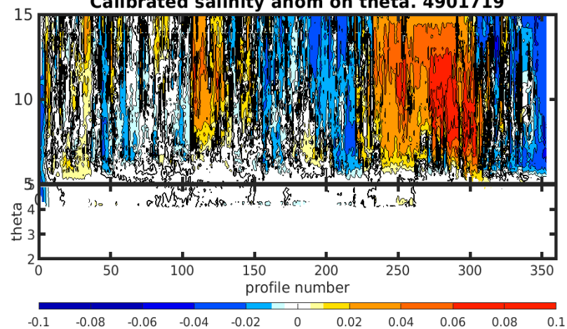
Calibrated salinity anom on theta. 4901719
