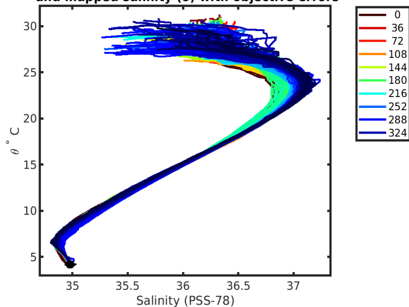
4901719 uncalibrated float data (-) and mapped salinity (o) with objective errors
