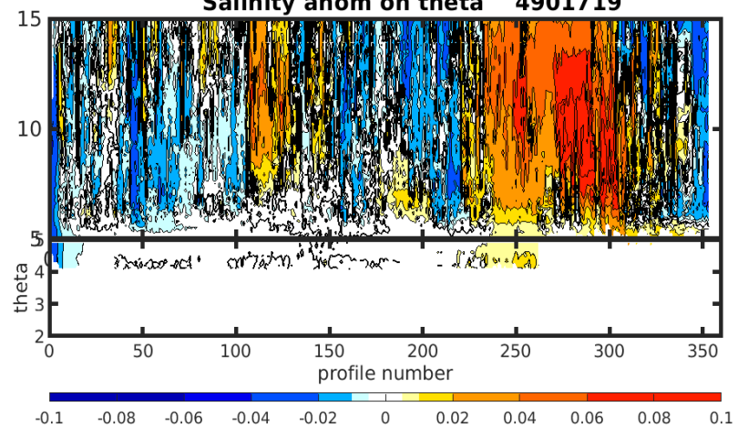
Salinity anom on theta 4901719
