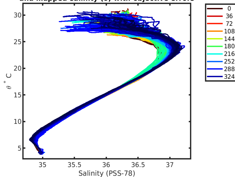
4901719 calibrated float data (-) and mapped salinity (o) with objective errors
