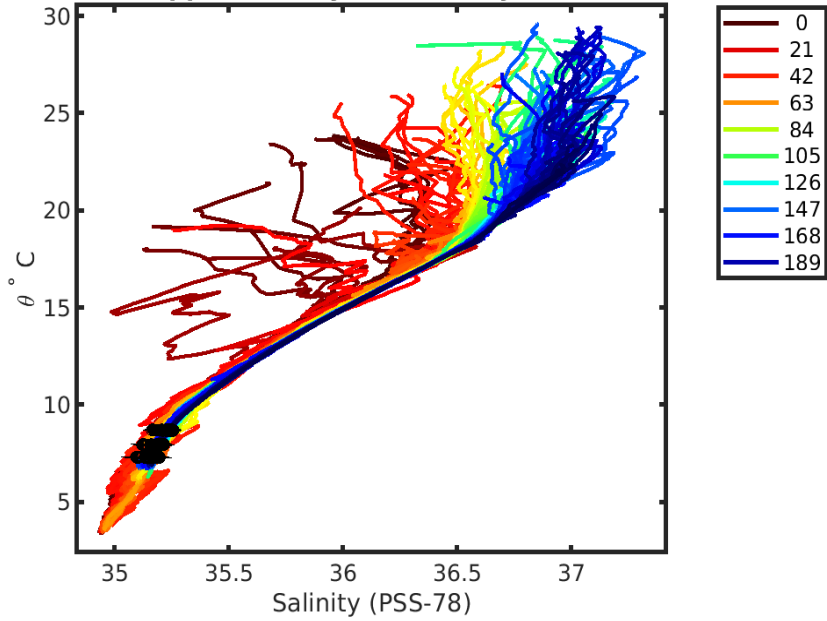
4901705 uncalibrated float data (-) and mapped salinity (o) with objective errors
