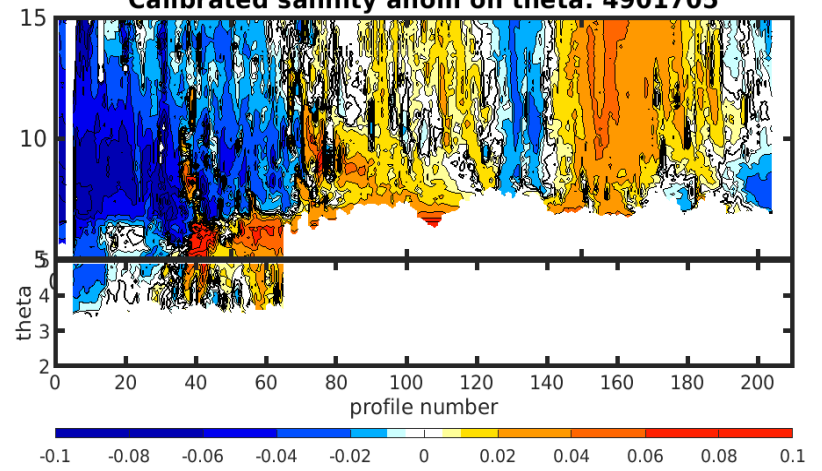
Calibrated salinity anom on theta. 4901705
