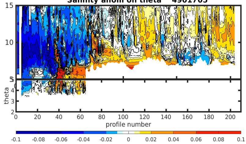
Salinity anom on theta 4901705
