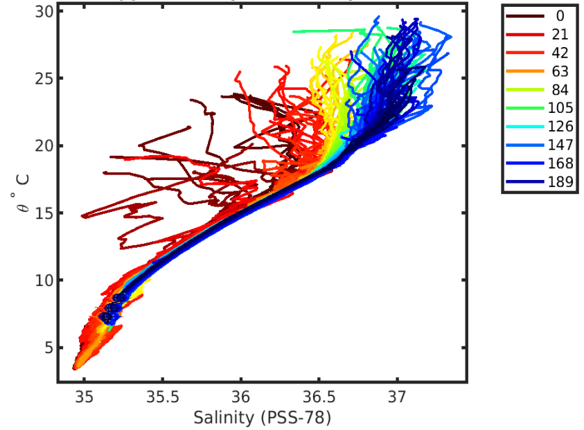
4901705 calibrated float data (-) and mapped salinity (o) with objective errors
