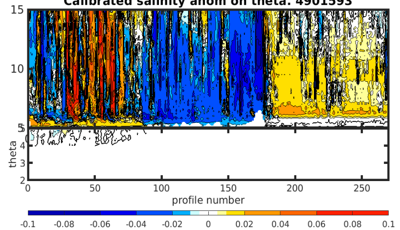
Calibrated salinity anom on theta. 4901593
