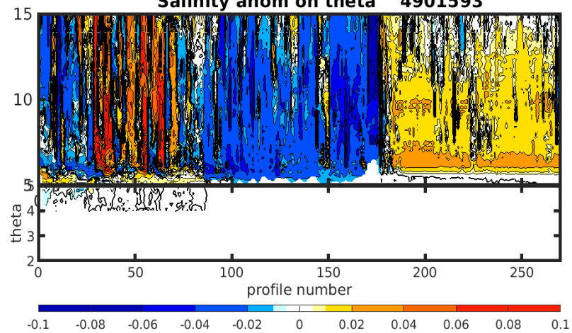
Salinity anom on theta 4901593
