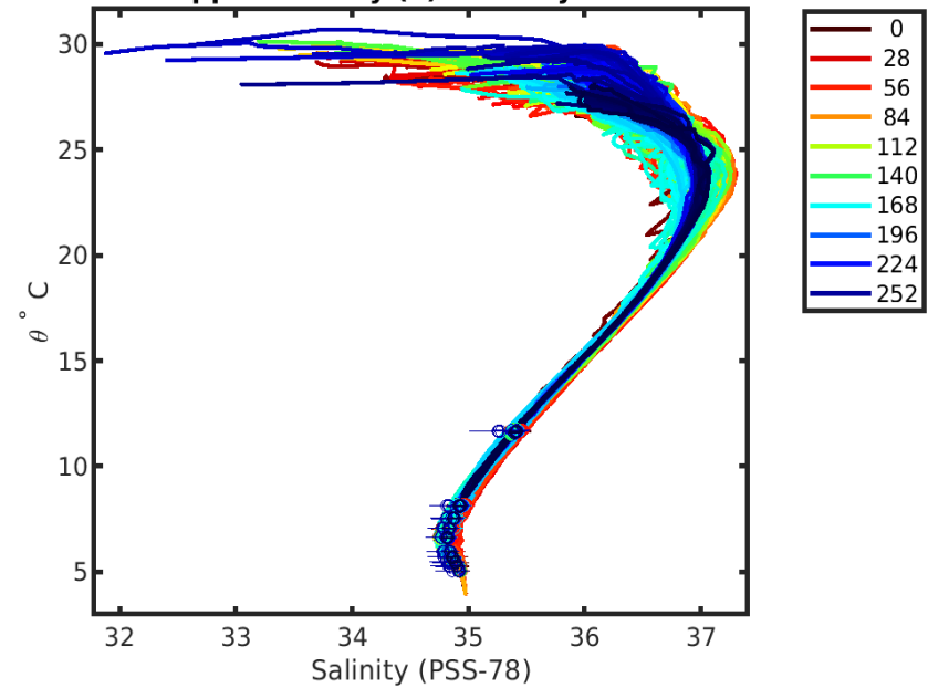
4901593 calibrated float data (-) and mapped salinity (o) with objective errors
