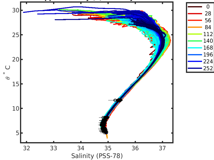
4901593 uncalibrated float data (-) and mapped salinity (o) with objective errors
