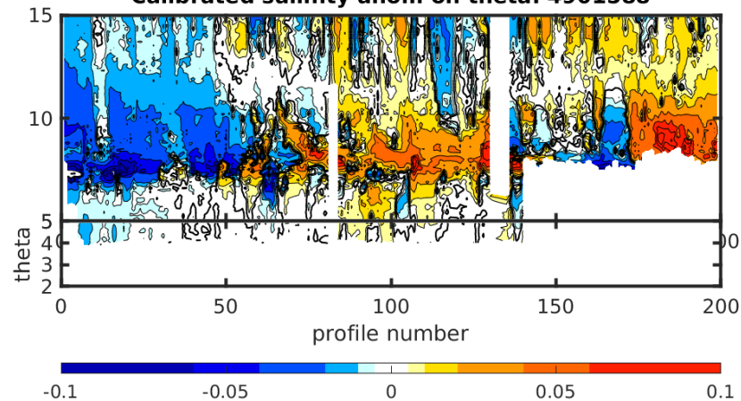
Calibrated salinity anom on theta. 4901588
