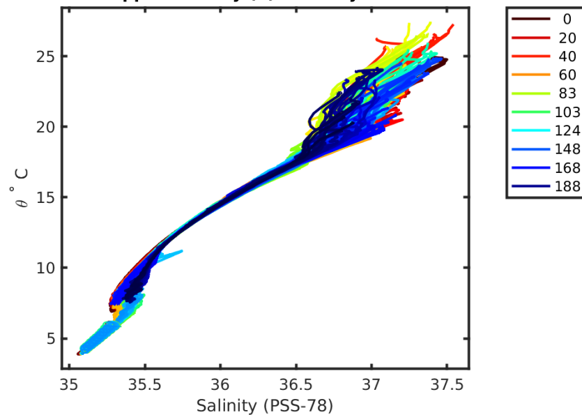
4901588 calibrated float data (-) and mapped salinity (o) with objective errors
