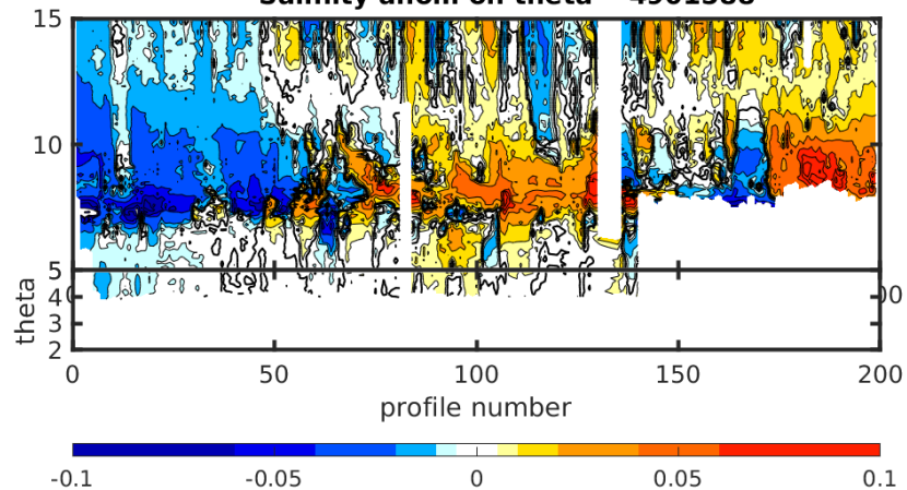
Salinity anom on theta 4901588
