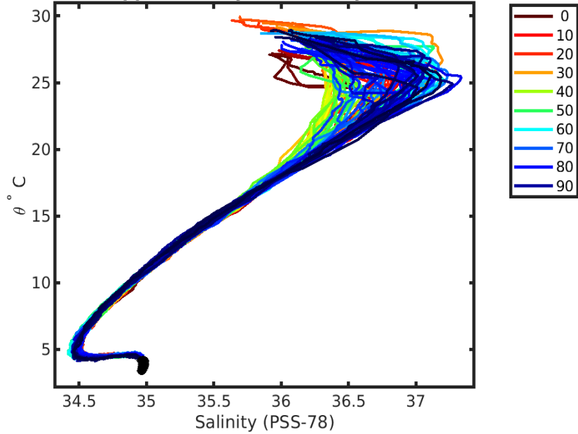
3902169 uncalibrated float data (-) and mapped salinity (o) with objective errors
