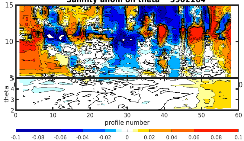
Salinity anom on theta 3902164
