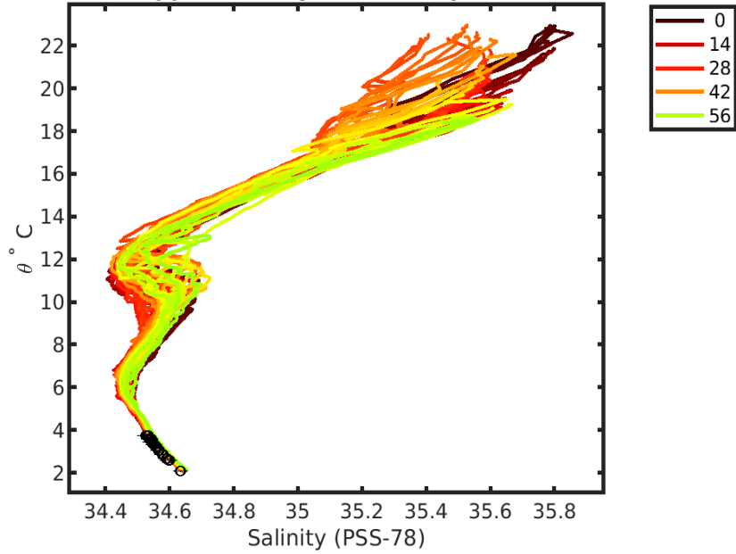
3902164 uncalibrated float data (-) and mapped salinity (o) with objective errors
