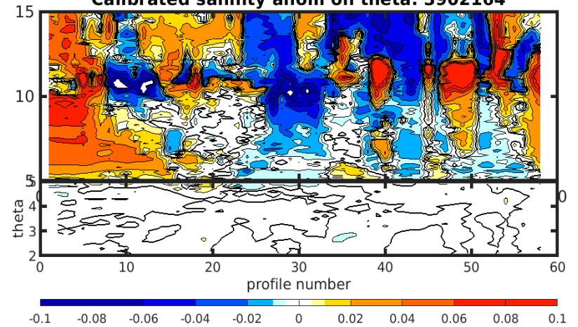
Calibrated salinity anom on theta. 3902164
