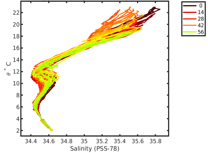
3902164 calibrated float data (-) and mapped salinity (o) with objective errors
