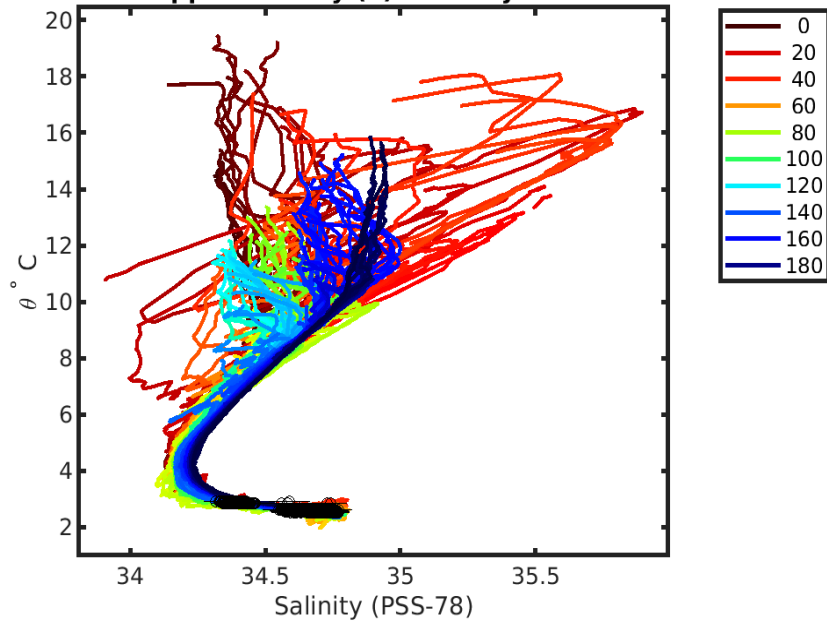
3901834 uncalibrated float data (-) and mapped salinity (o) with objective errors
