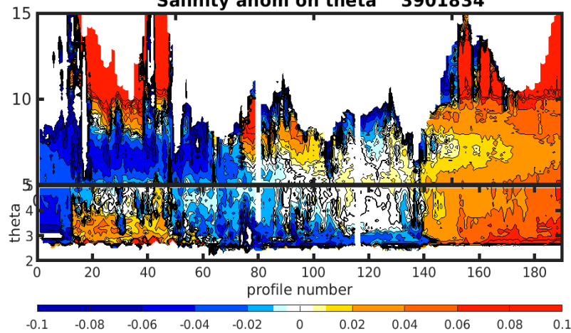
Salinity anom on theta 3901834
