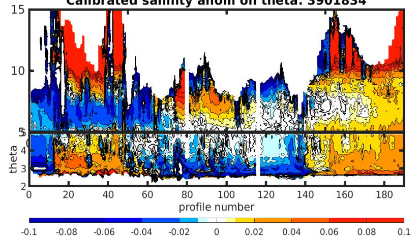
Calibrated salinity anom on theta. 3901834
