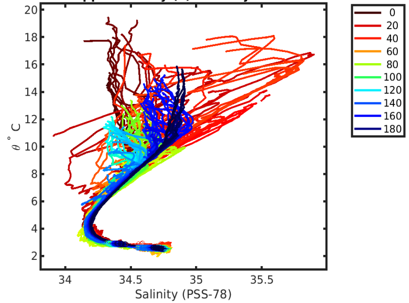
3901834 calibrated float data (-) and mapped salinity (o) with objective errors
