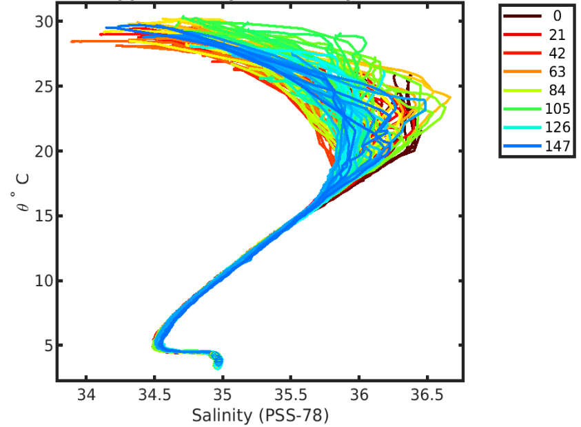
3901821 calibrated float data (-) and mapped salinity (o) with objective errors
