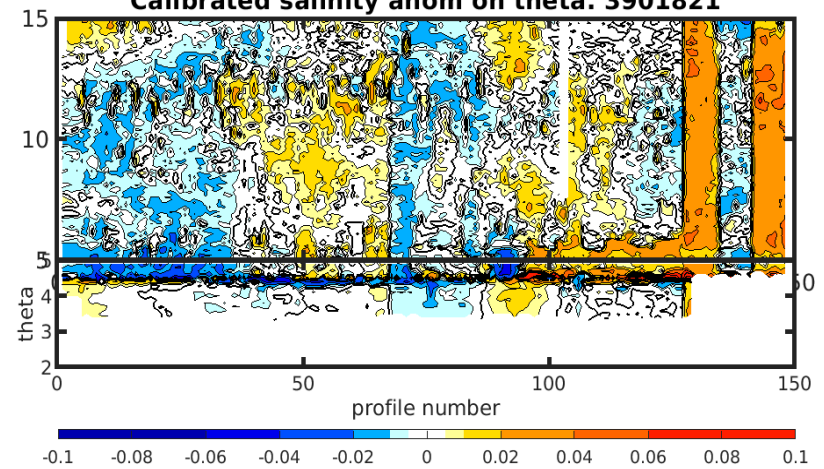
Calibrated salinity anom on theta. 3901821
