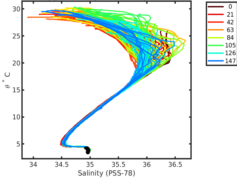
3901821 uncalibrated float data (-) and mapped salinity (o) with objective errors
