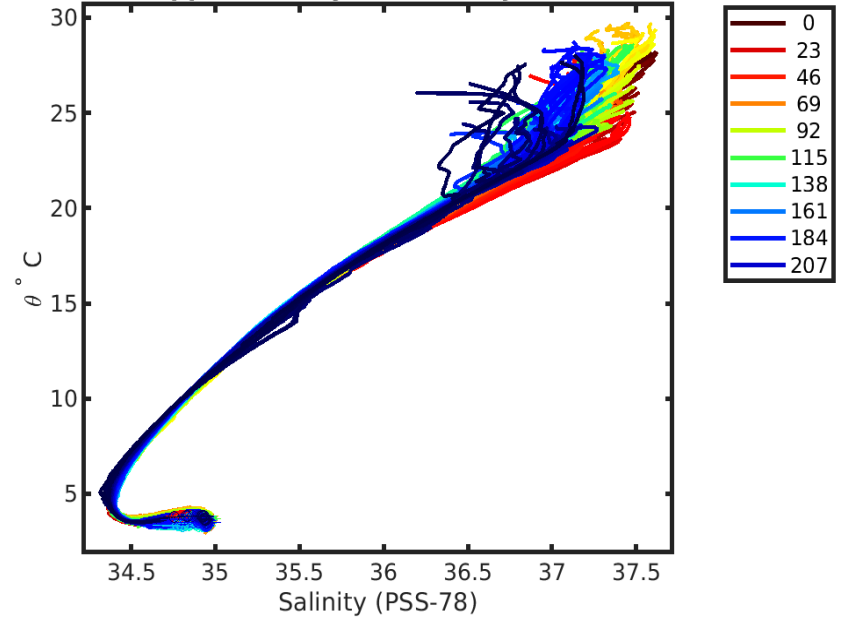
3901237 calibrated float data (-) and mapped salinity (o) with objective errors
