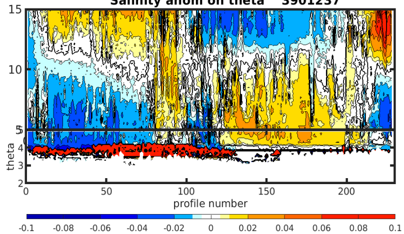
Salinity anom on theta 3901237
