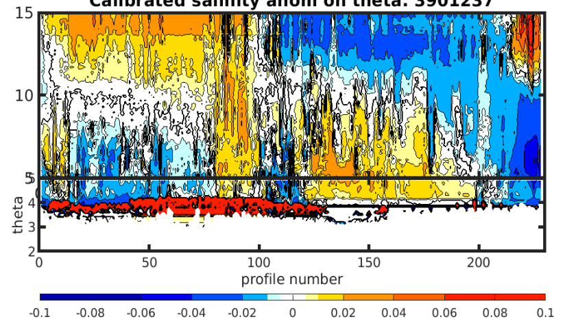
Calibrated salinity anom on theta. 3901237
