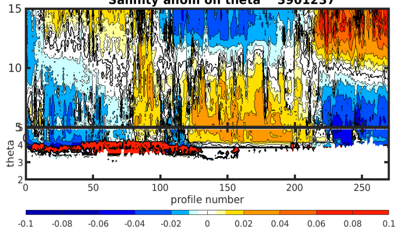
Salinity anom on theta 3901237
