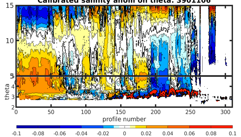
Calibrated salinity anom on theta. 3901106
