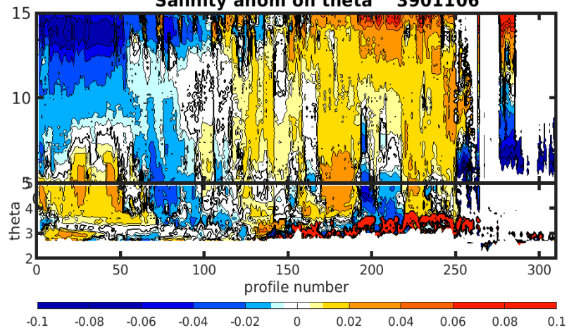
Salinity anom on theta 3901106
