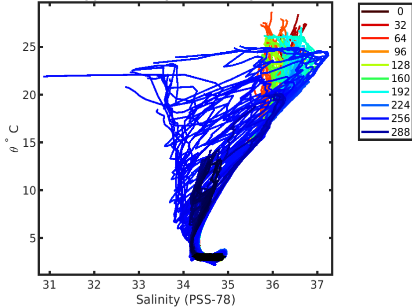
3901106 uncalibrated float data (-) and mapped salinity (o) with objective errors
