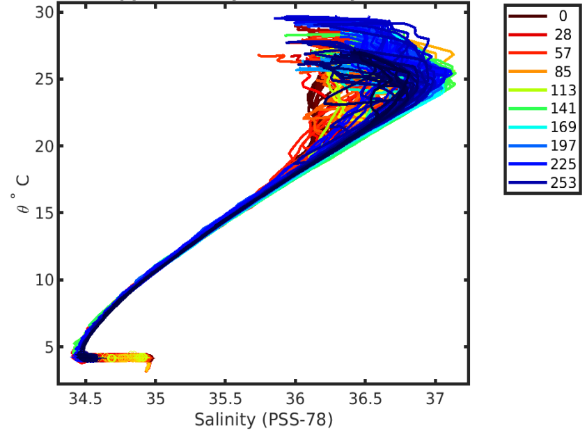
3901039 calibrated float data (-) and mapped salinity (o) with objective errors
