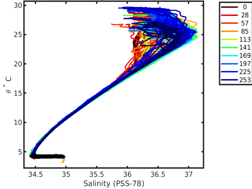
3901039 uncalibrated float data (-) and mapped salinity (o) with objective errors
