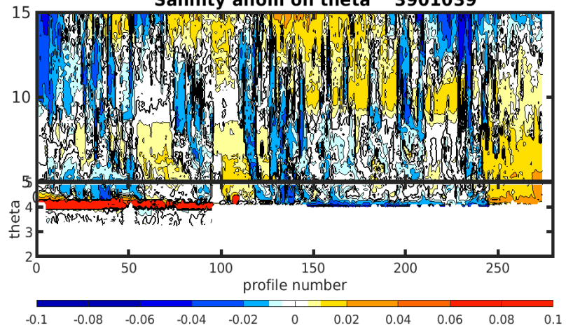
Salinity anom on theta 3901039
