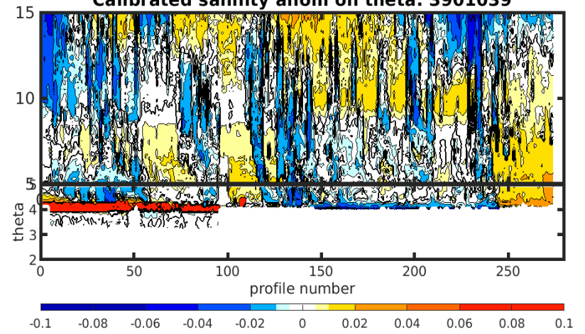
Calibrated salinity anom on theta. 3901039
