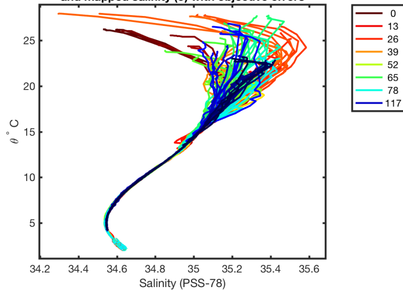
3900837 calibrated float data (-) and mapped salinity (o) with objective errors
