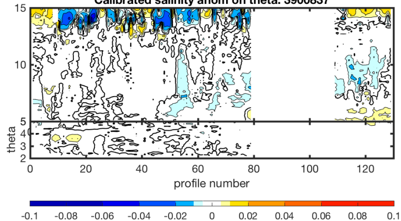
Calibrated salinity anom on theta. 3900837
