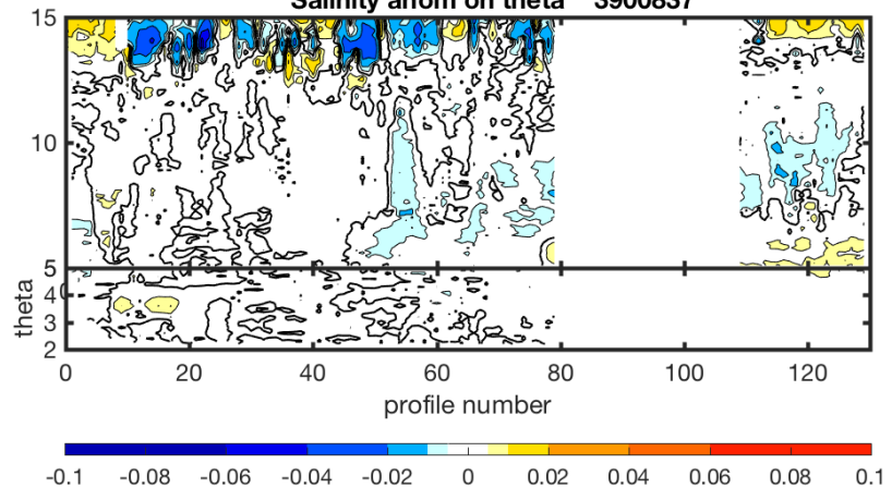
Salinity anom on theta 3900837
