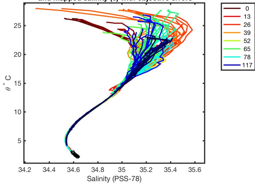
3900837 uncalibrated float data (-) and mapped salinity (o) with objective errors
