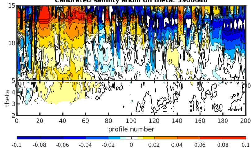
Calibrated salinity anom on theta. 3900648
