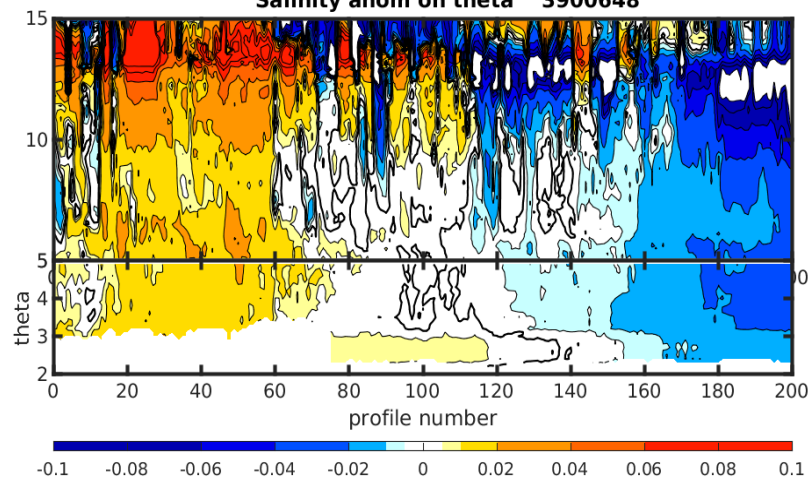
Salinity anom on theta 3900648
