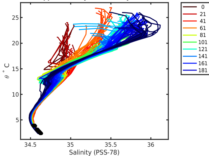
3900648 uncalibrated float data (-) and mapped salinity (o) with objective errors
