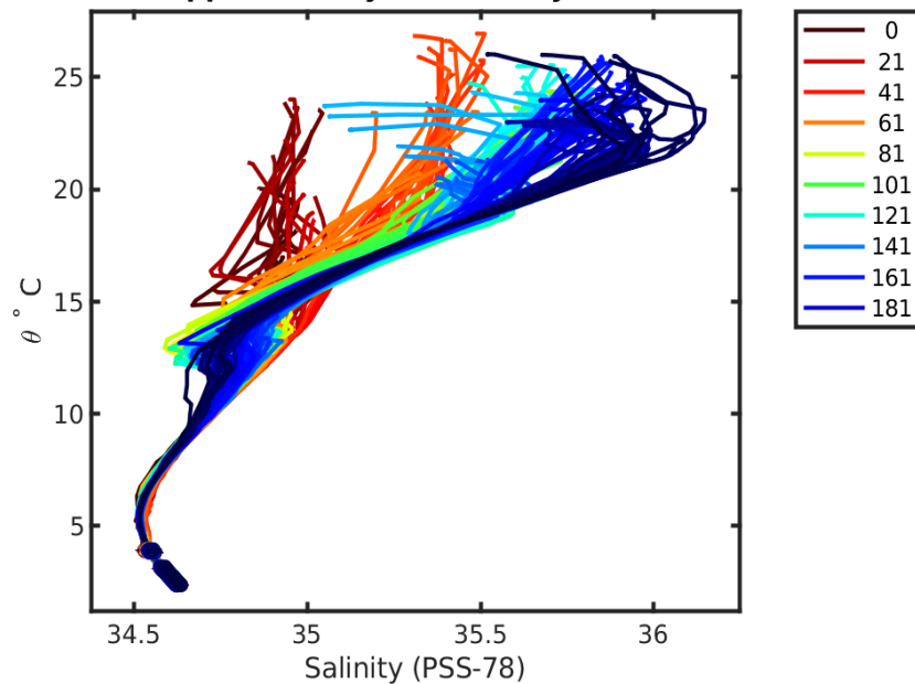
3900648 calibrated float data (-) and mapped salinity (o) with objective errors
