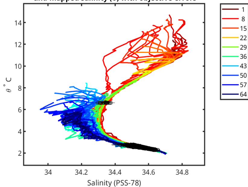
2903937 uncalibrated float data (-) and mapped salinity (o) with objective errors
