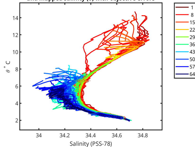
2903937 calibrated float data (-) and mapped salinity (o) with objective errors
