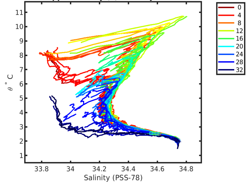
1902523 calibrated float data (-) and mapped salinity (o) with objective errors
