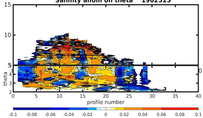
Salinity anom on theta 1902523
