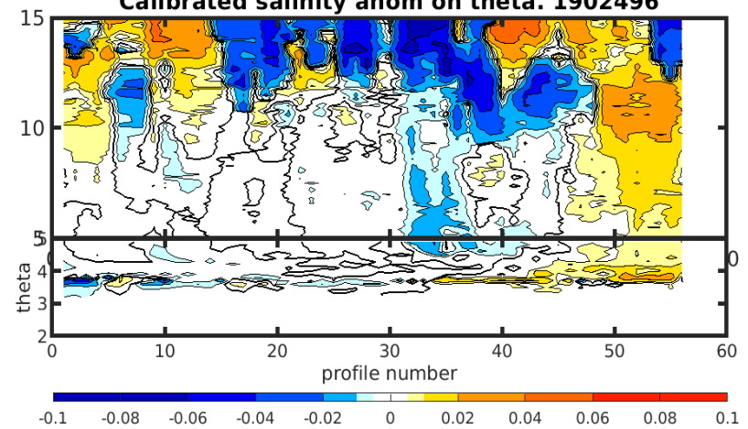
Calibrated salinity anom on theta. 1902496
