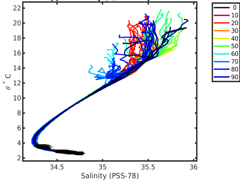
1902486 uncalibrated float data (-) and mapped salinity (o) with objective errors
