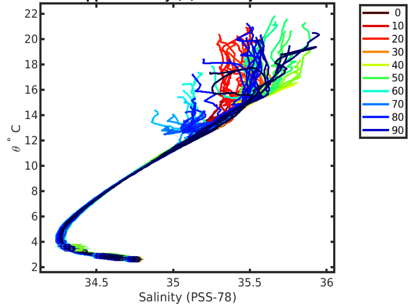
1902486 calibrated float data (-) and mapped salinity (o) with objective errors
