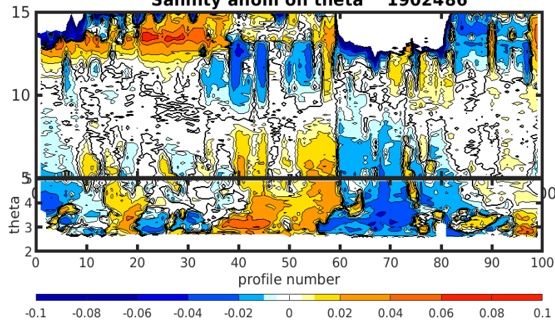
Salinity anom on theta 1902486
