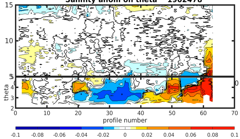
Salinity anom on theta 1902478
