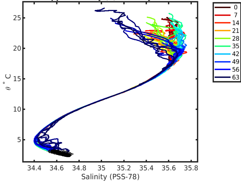
1902478 uncalibrated float data (-) and mapped salinity (o) with objective errors
