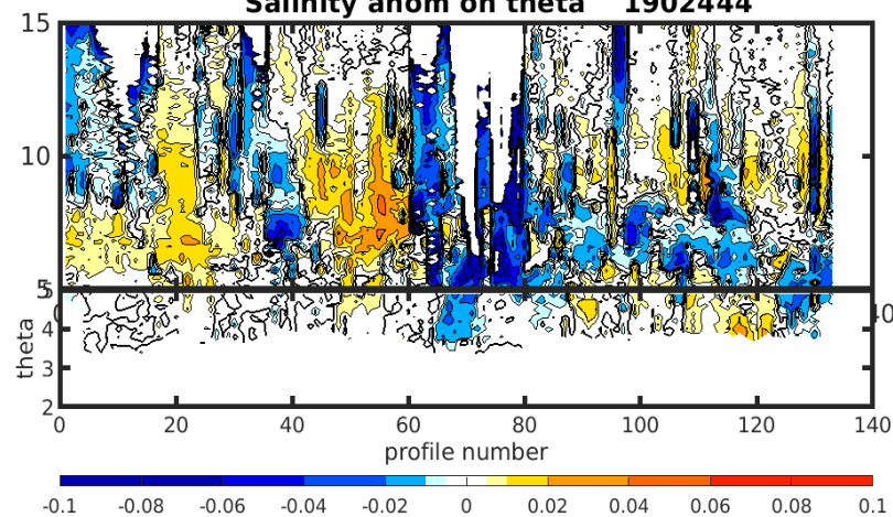
Salinity anom on theta 1902444
