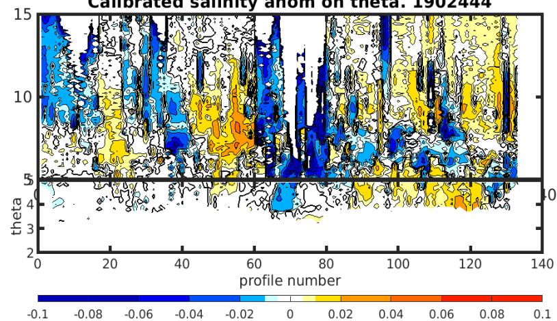
Calibrated salinity anom on theta. 1902444
