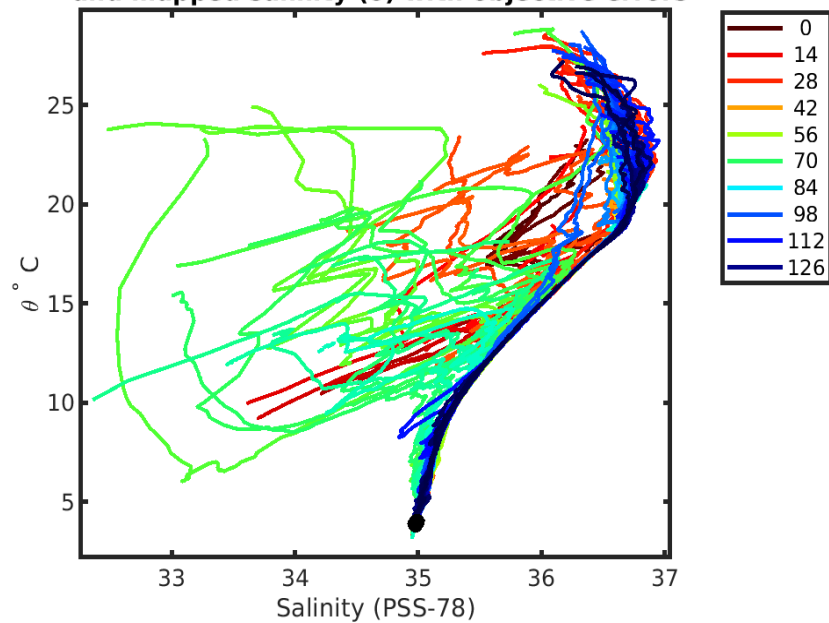
1902444 uncalibrated float data (-) and mapped salinity (o) with objective errors
