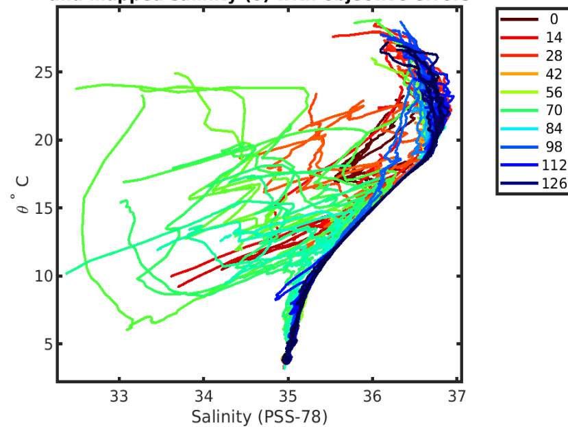
1902444 calibrated float data (-) and mapped salinity (o) with objective errors
