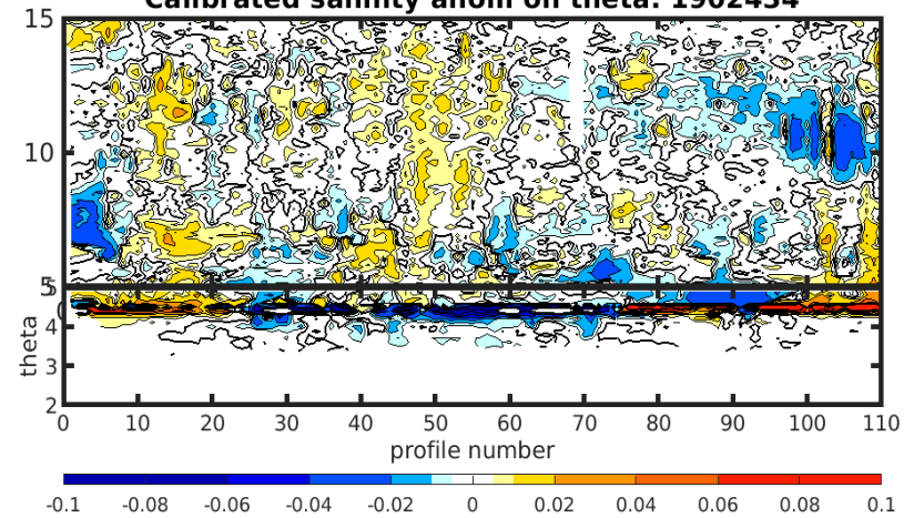
Calibrated salinity anom on theta. 1902434
