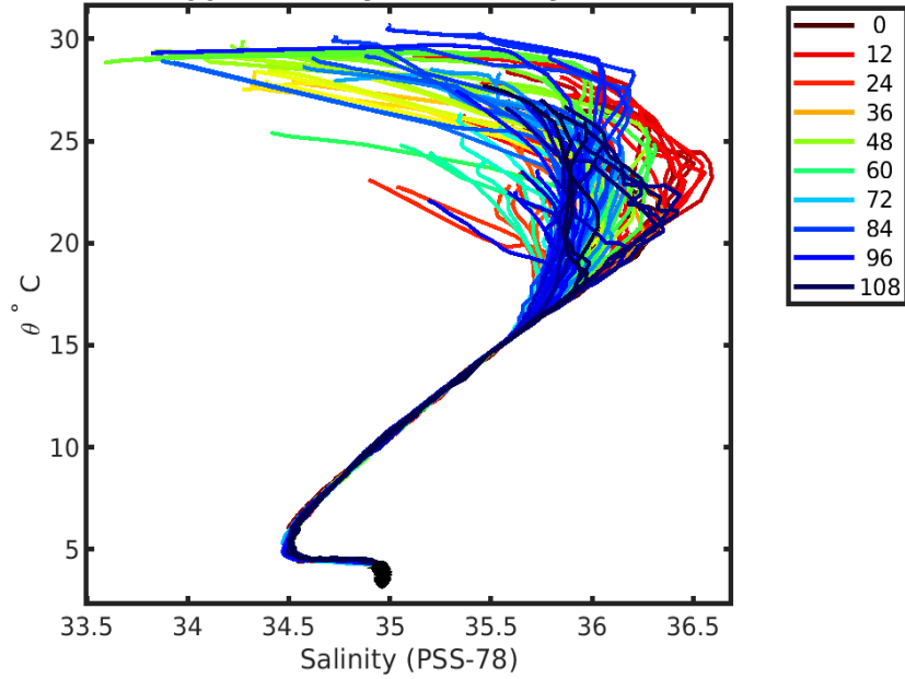
1902434 uncalibrated float data (-) and mapped salinity (o) with objective errors
