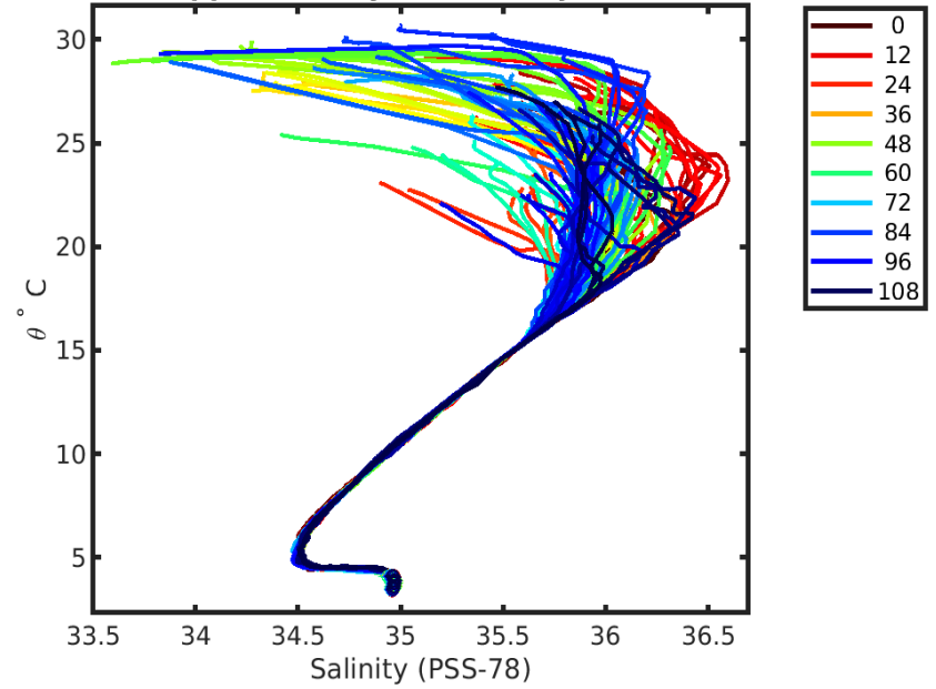
1902434 calibrated float data (-) and mapped salinity (o) with objective errors
