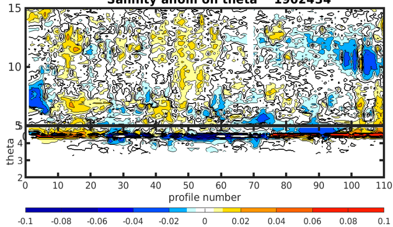
Salinity anom on theta 1902434
