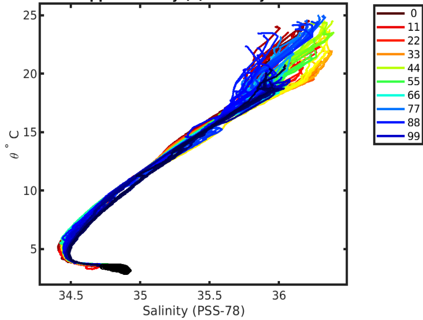
1902424 uncalibrated float data (-) and mapped salinity (o) with objective errors
