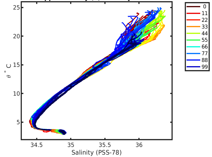
1902424 calibrated float data (-) and mapped salinity (o) with objective errors
