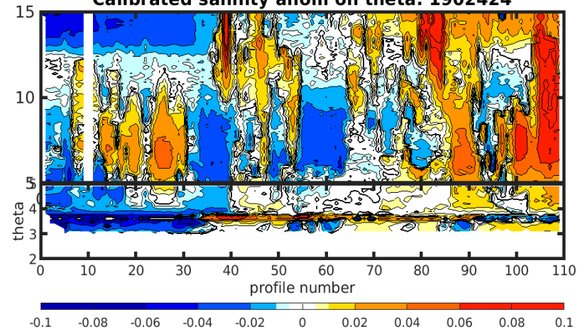
Calibrated salinity anom on theta. 1902424
