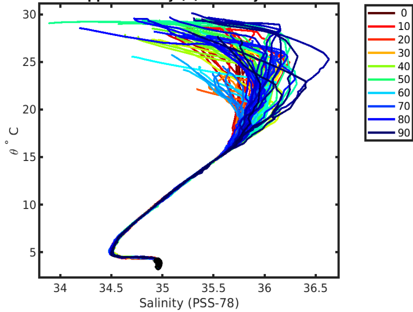
1902420 uncalibrated float data (-) and mapped salinity (o) with objective errors
