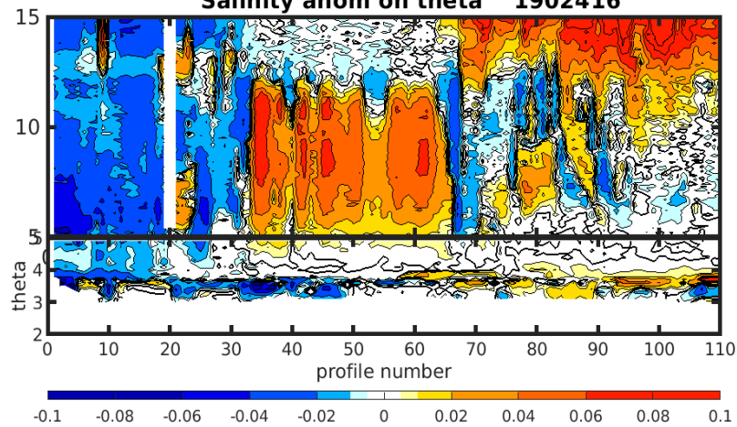
Salinity anom on theta 1902416
