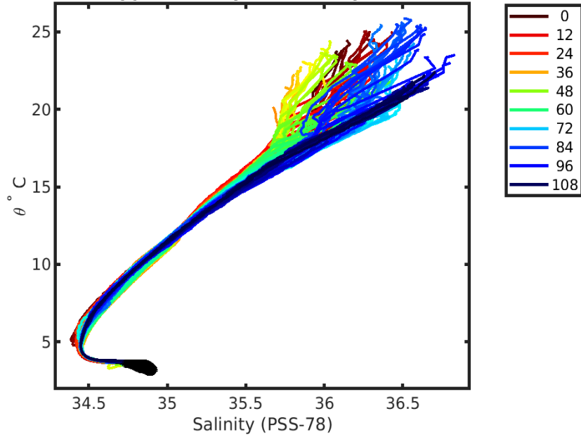
1902416 uncalibrated float data (-) and mapped salinity (o) with objective errors
