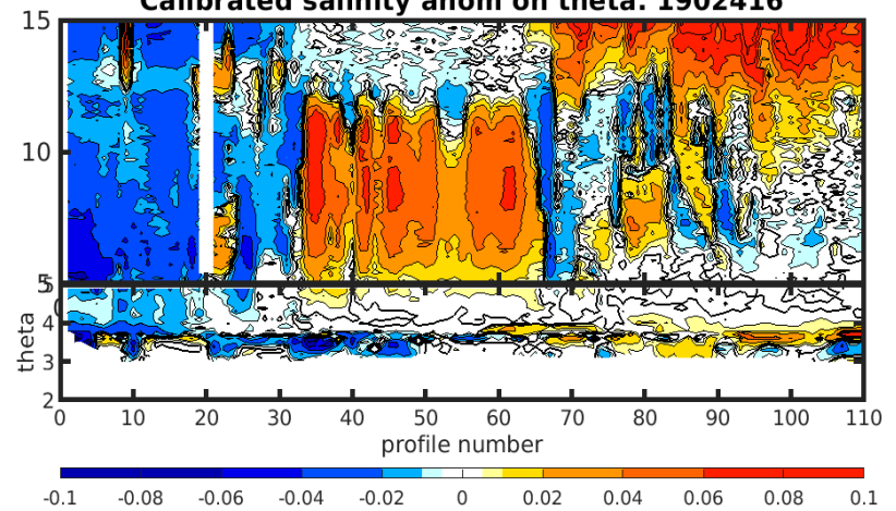
Calibrated salinity anom on theta. 1902416
