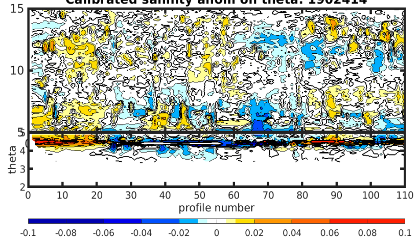
Calibrated salinity anom on theta. 1902414
