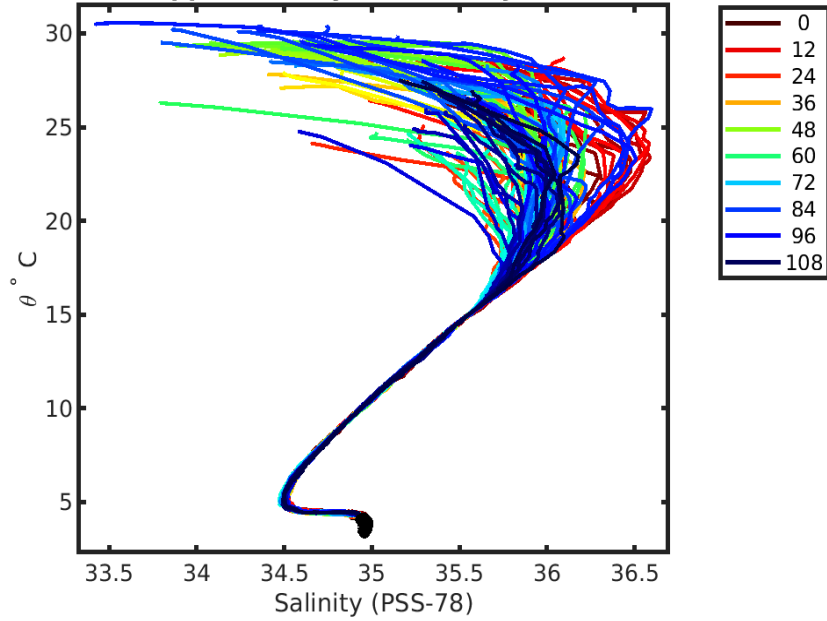
1902414 uncalibrated float data (-) and mapped salinity (o) with objective errors
