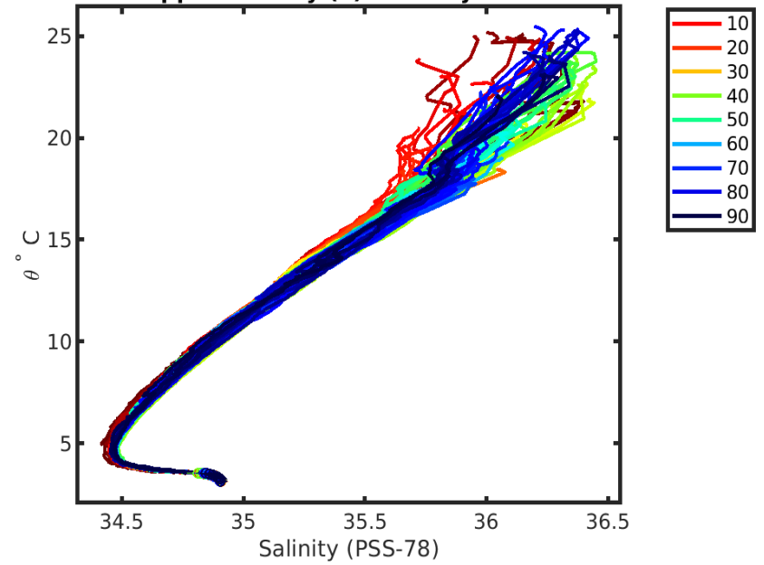
1902409 calibrated float data (-) and mapped salinity (o) with objective errors
