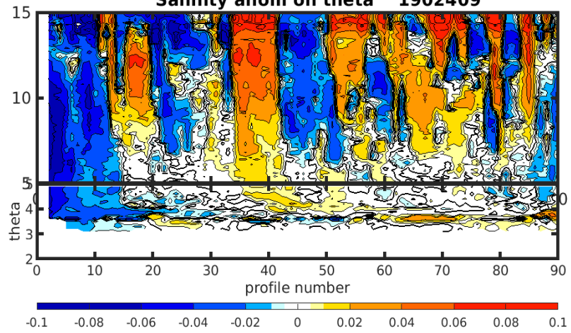
Salinity anom on theta 1902409
