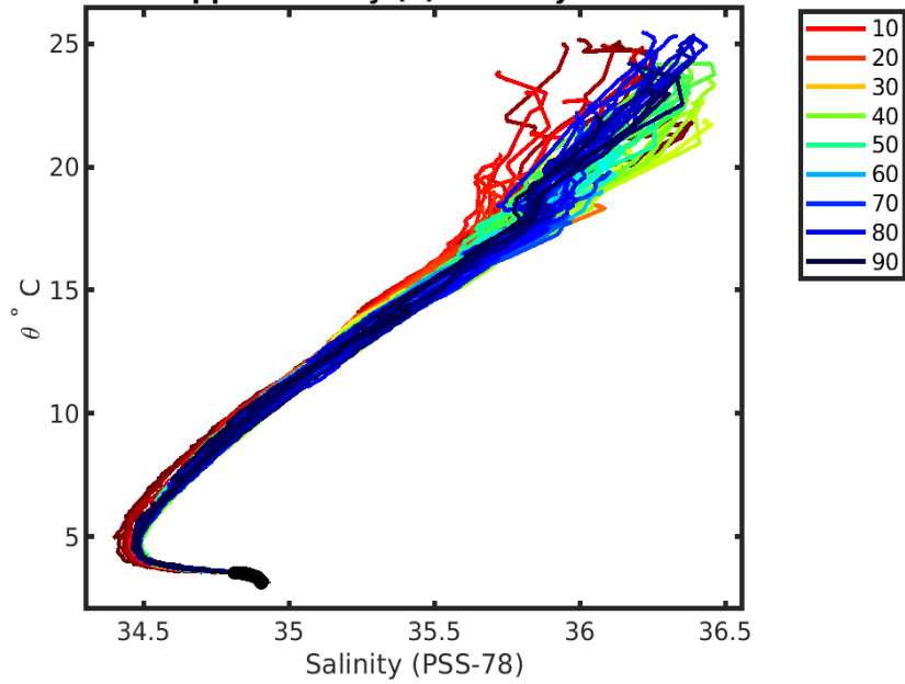
1902409 uncalibrated float data (-) and mapped salinity (o) with objective errors
