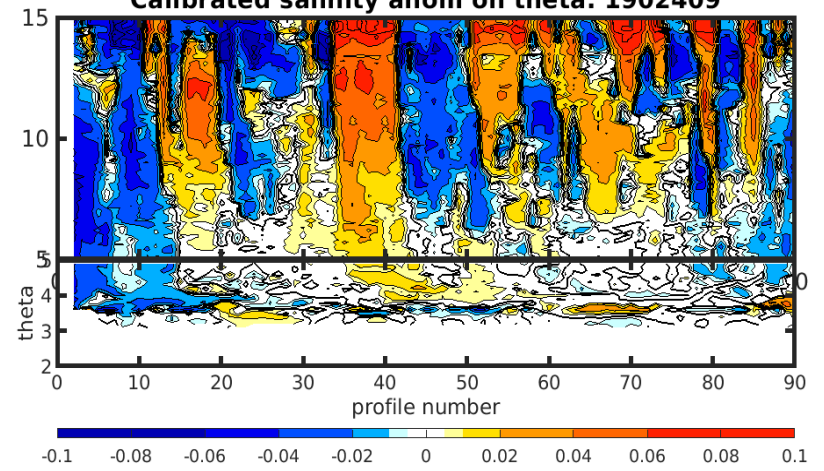
Calibrated salinity anom on theta. 1902409
