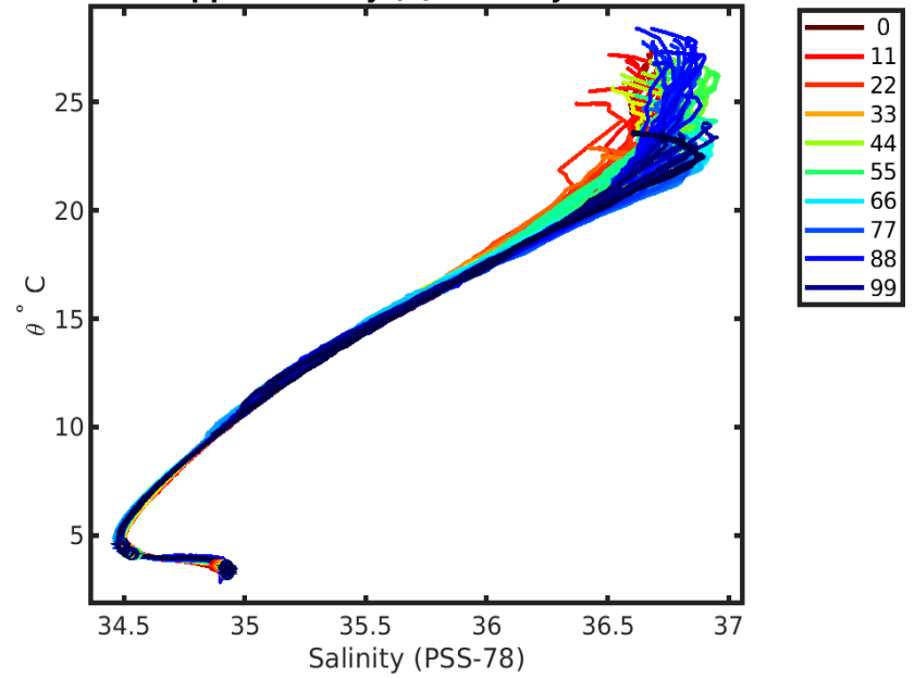
1902405 calibrated float data (-) and mapped salinity (o) with objective errors
