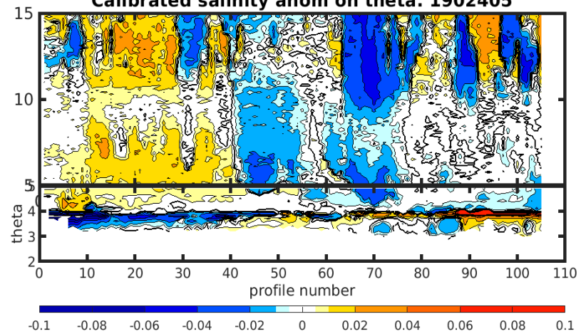
Calibrated salinity anom on theta. 1902405
