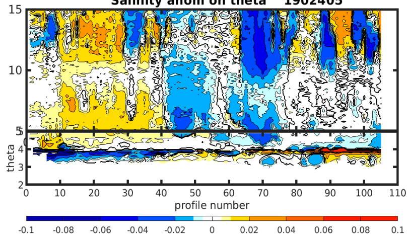
Salinity anom on theta 1902405
