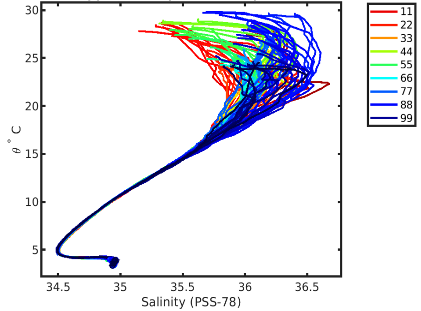
1902399 calibrated float data (-) and mapped salinity (o) with objective errors
