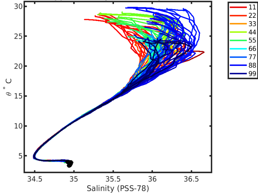
1902399 uncalibrated float data (-) and mapped salinity (o) with objective errors
