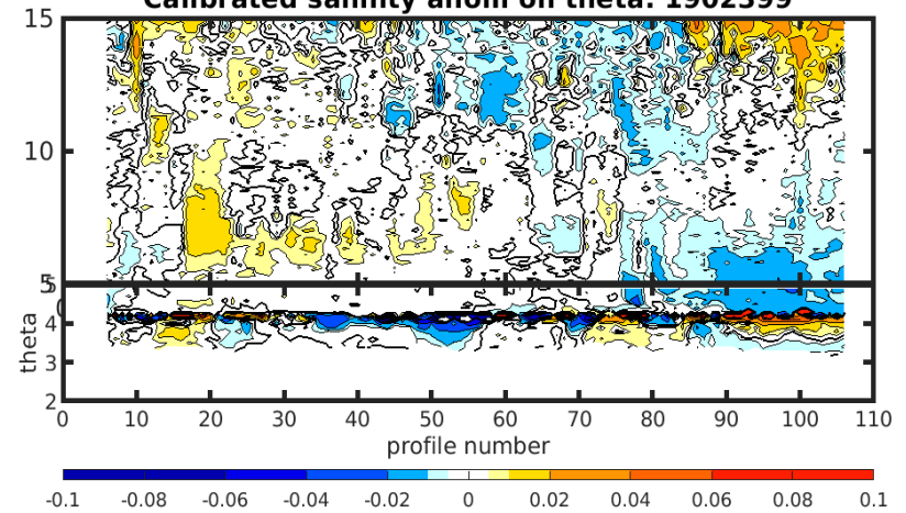
Calibrated salinity anom on theta. 1902399
