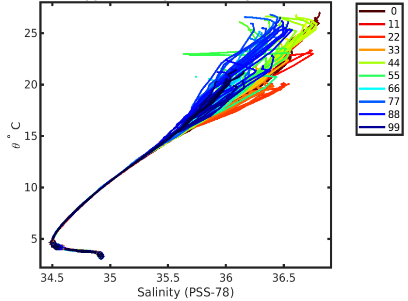
1902329 calibrated float data (-) and mapped salinity (o) with objective errors
