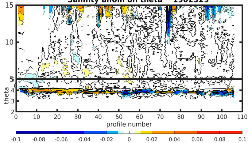
Salinity anom on theta 1902329
