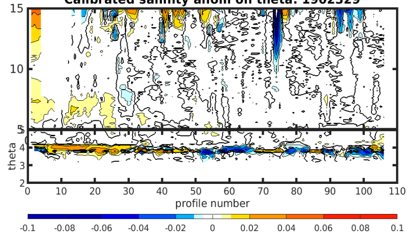
Calibrated salinity anom on theta. 1902329
