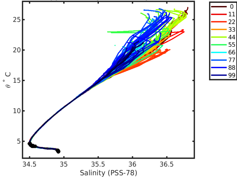
1902329 uncalibrated float data (-) and mapped salinity (o) with objective errors
