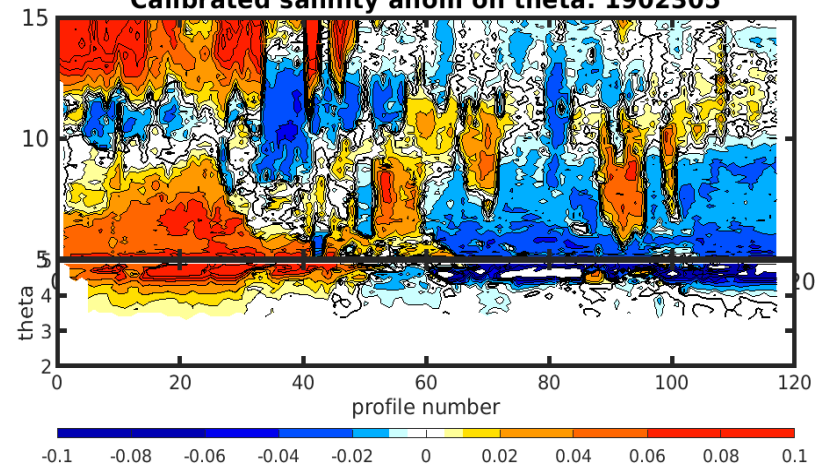
Calibrated salinity anom on theta. 1902305
