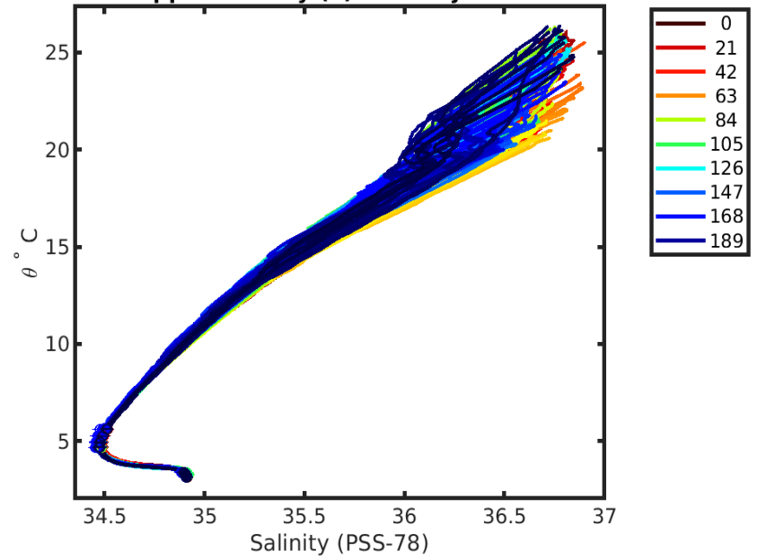
1901822 calibrated float data (-) and mapped salinity (o) with objective errors
