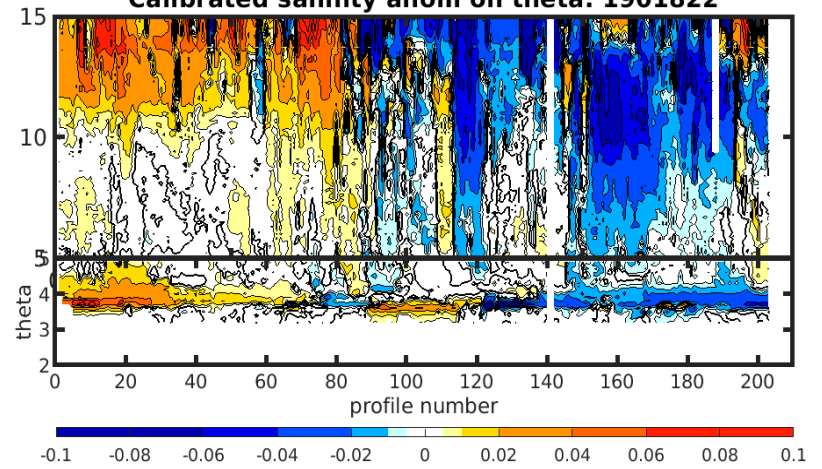
Calibrated salinity anom on theta. 1901822
