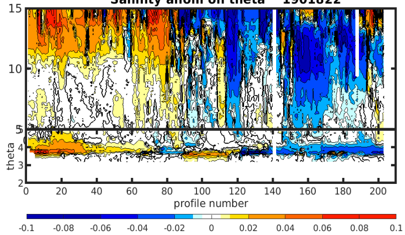
Salinity anom on theta 1901822
