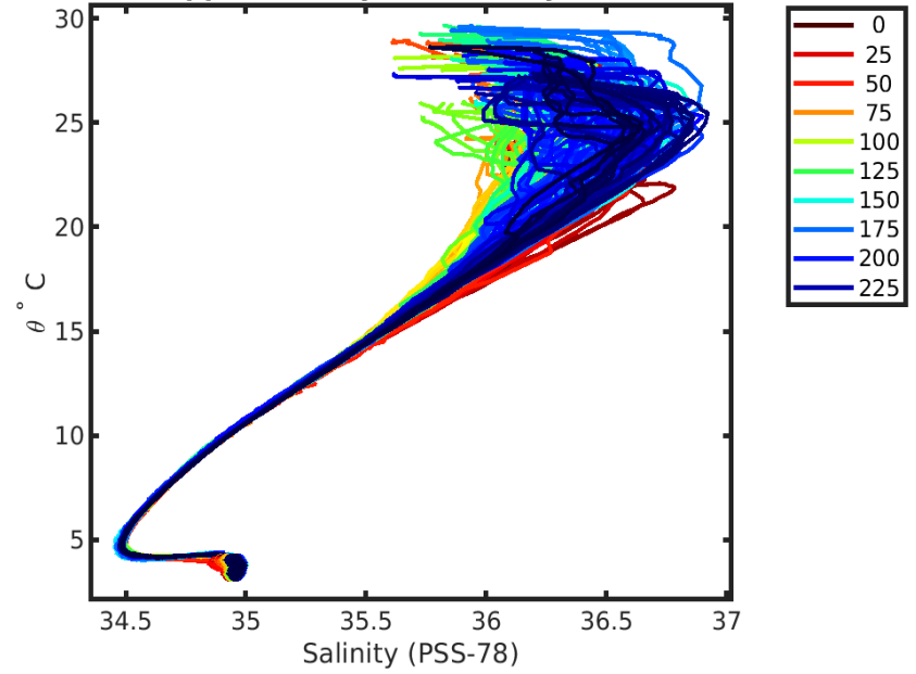
1901807 calibrated float data (-) and mapped salinity (o) with objective errors
