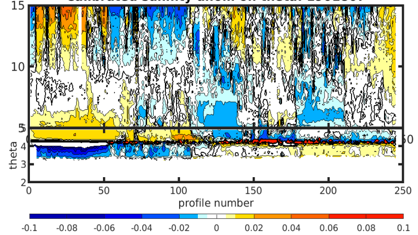
Calibrated salinity anom on theta. 1901807
