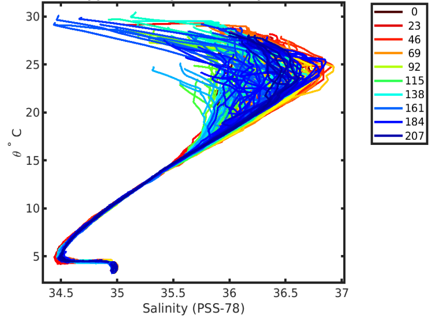
1901806 calibrated float data (-) and mapped salinity (o) with objective errors
