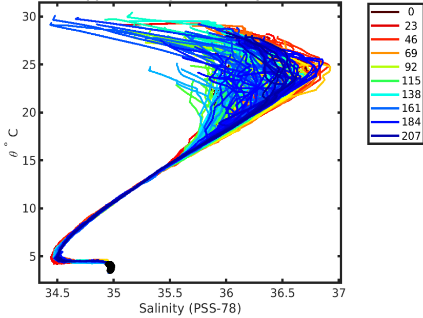
1901806 uncalibrated float data (-) and mapped salinity (o) with objective errors
