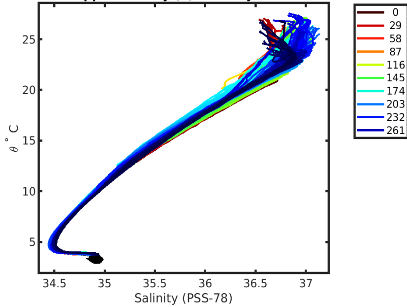
1901784 uncalibrated float data (-) and mapped salinity (o) with objective errors
