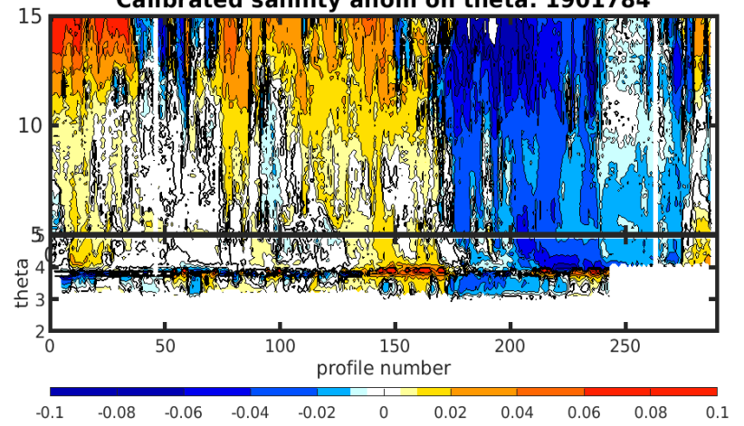
Calibrated salinity anom on theta. 1901784
