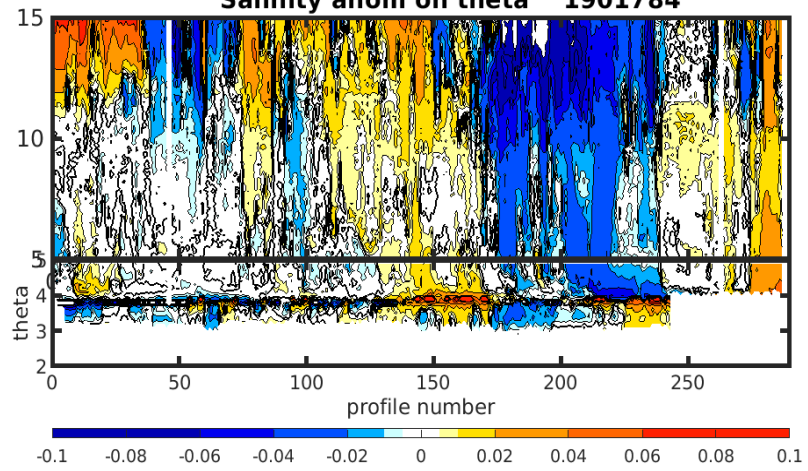
Salinity anom on theta 1901784
