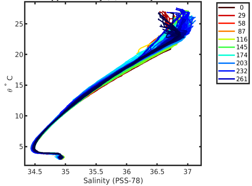
1901784 calibrated float data (-) and mapped salinity (o) with objective errors
