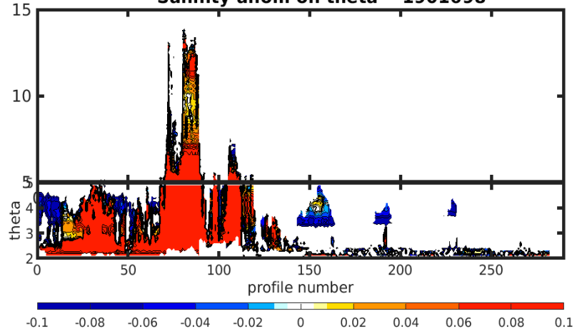
Salinity anom on theta 1901698
