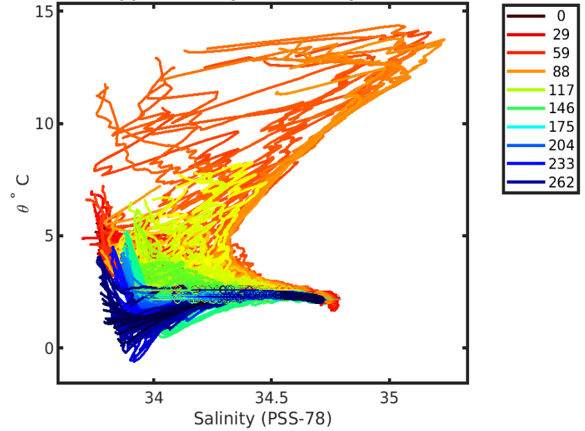
1901698 calibrated float data (-) and mapped salinity (o) with objective errors
