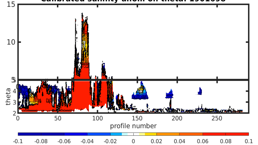
Calibrated salinity anom on theta. 1901698
