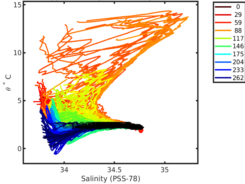
1901698 uncalibrated float data (-) and mapped salinity (o) with objective errors
