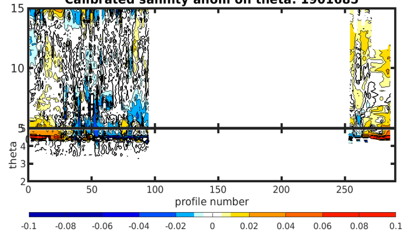
Calibrated salinity anom on theta. 1901685
