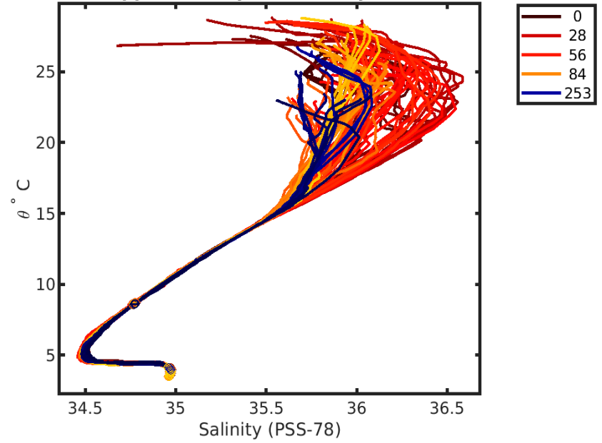
1901685 calibrated float data (-) and mapped salinity (o) with objective errors
