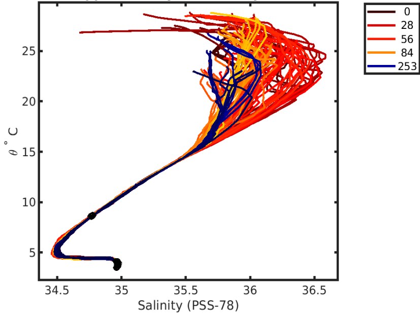
1901685 uncalibrated float data (-) and mapped salinity (o) with objective errors
