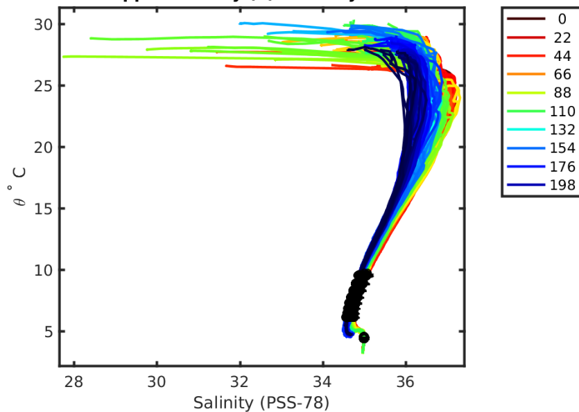
1901672 uncalibrated float data (-) and mapped salinity (o) with objective errors
