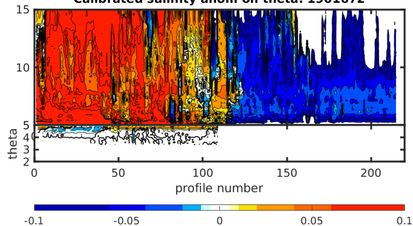
Calibrated salinity anom on theta. 1901672
