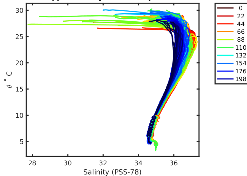
1901672 calibrated float data (-) and mapped salinity (o) with objective errors
