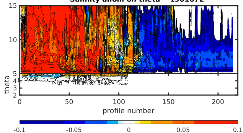
Salinity anom on theta 1901672
