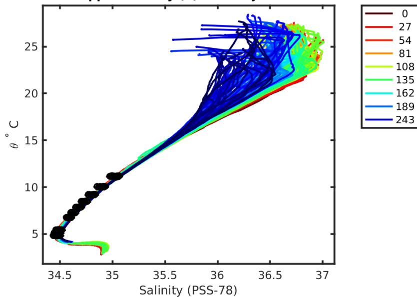
1901647 uncalibrated float data (-) and mapped salinity (o) with objective errors
