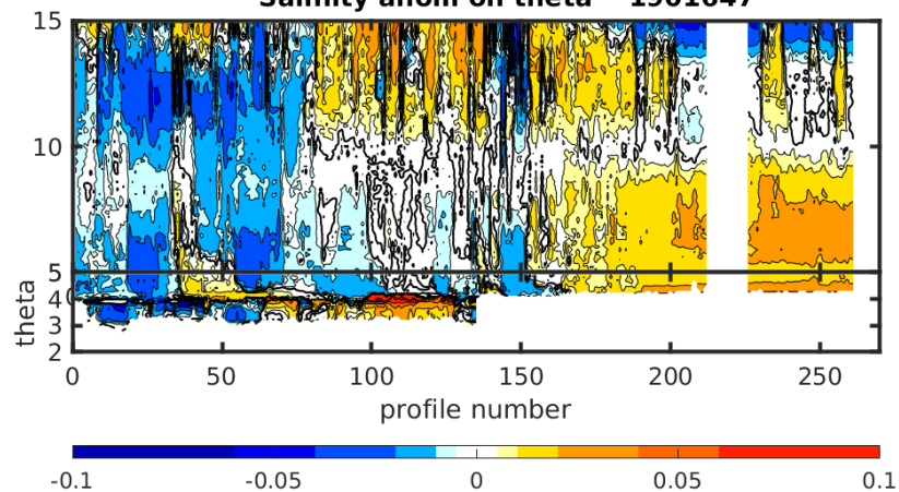
Salinity anom on theta 1901647
