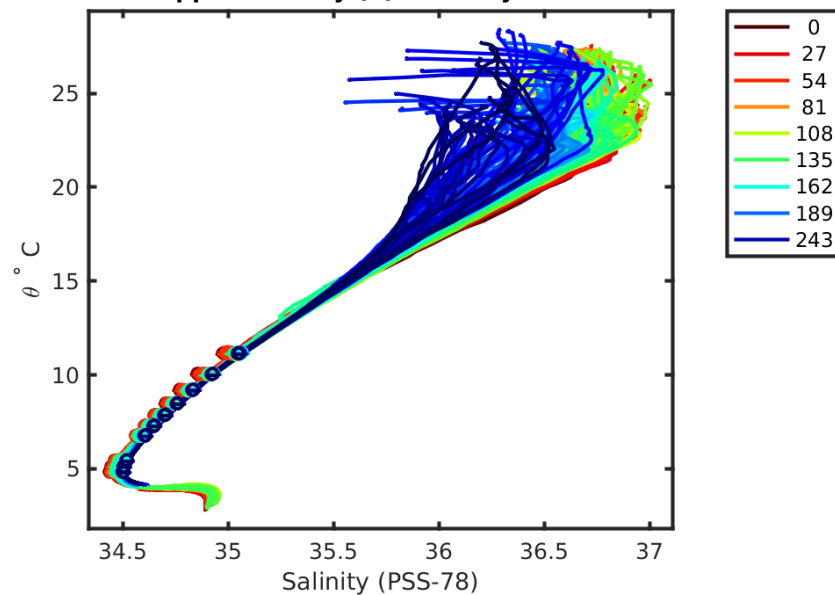
1901647 calibrated float data (-) and mapped salinity (o) with objective errors
