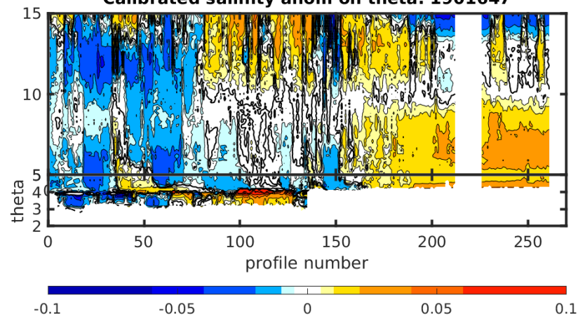
Calibrated salinity anom on theta. 1901647
