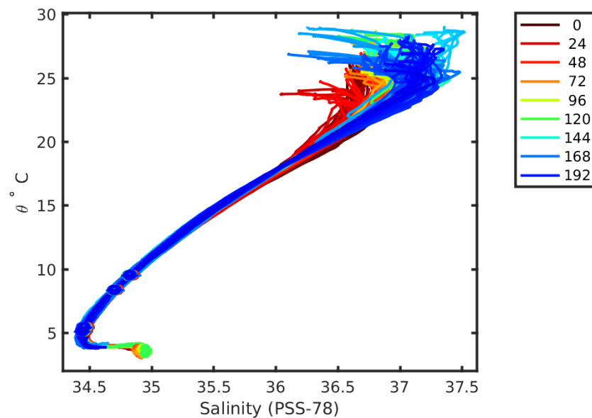
1901646 calibrated float data (-) and mapped salinity (o) with objective errors
