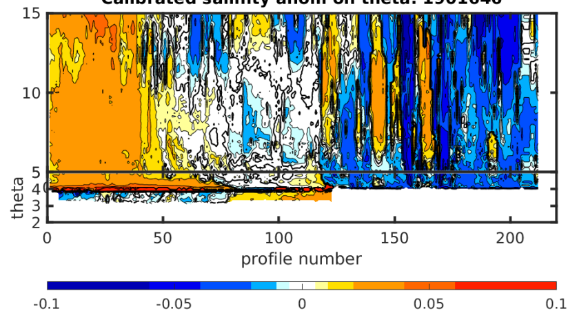
Calibrated salinity anom on theta. 1901646
