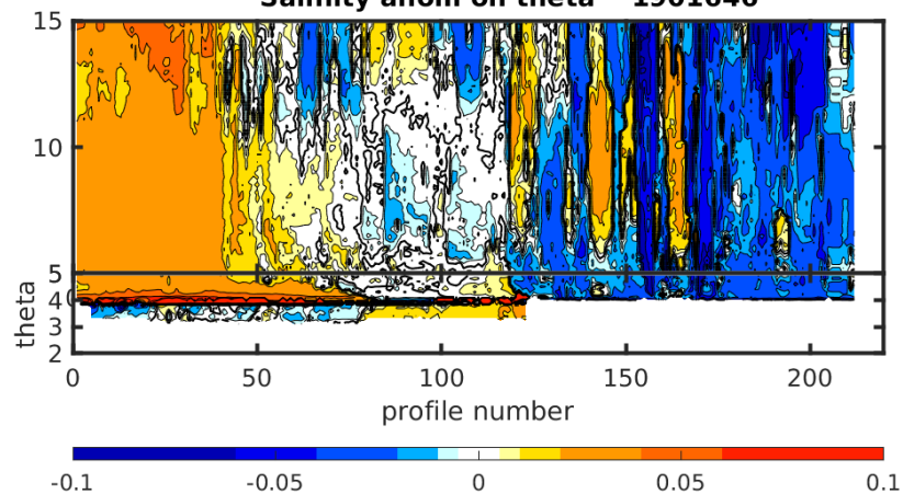
Salinity anom on theta 1901646
