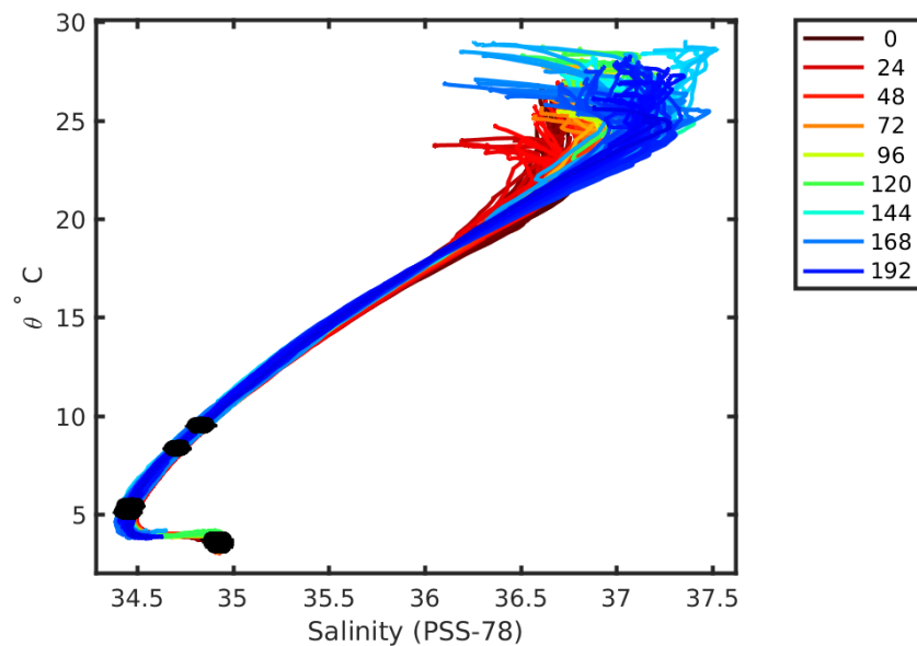
1901646 uncalibrated float data (-) and mapped salinity (o) with objective errors
