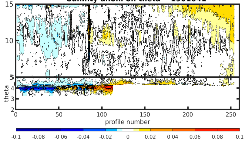
Salinity anom on theta 1901641
