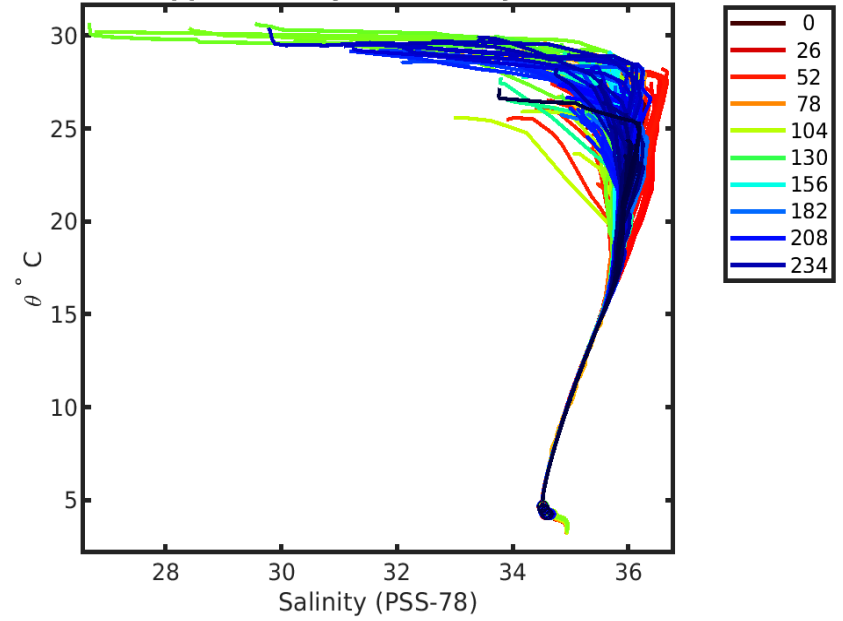
1901641 calibrated float data (-) and mapped salinity (o) with objective errors
