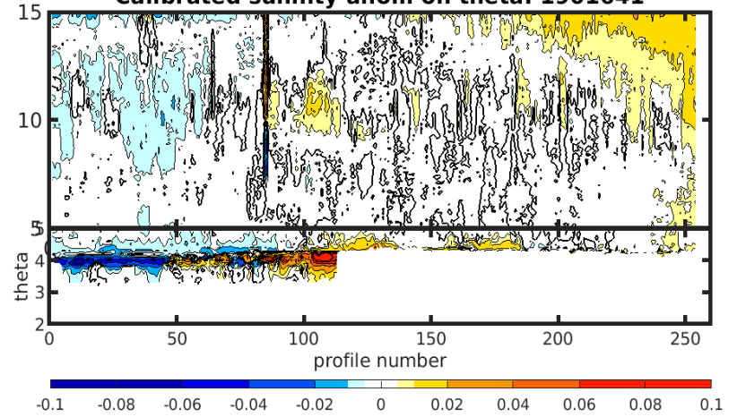
Calibrated salinity anom on theta. 1901641
